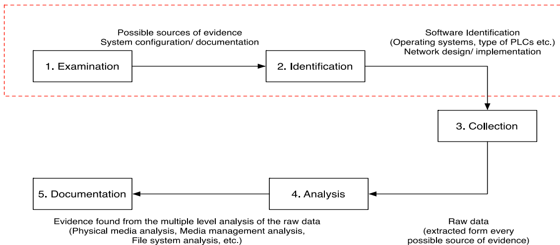
Fig 1. Ex post incident analysis process in SCADA systems.
