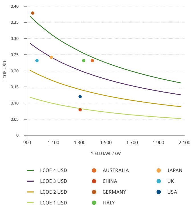
FIGURE 22: LCOE OF PV ELECTRICITY (USD) AS A FUNCTION OF SOLAR IRRADIANCE (kWh/kW/YEAR) & RETAIL PRICES IN 10 MAJOR MARKETS
