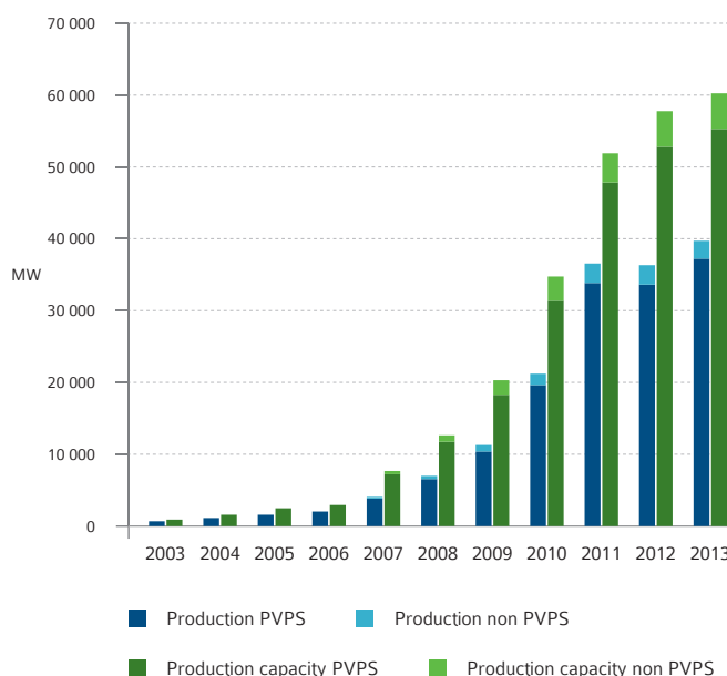
FIGURE 16: YEARLY PV MODULE PRODUCTION AND PRODUCTION CAPACITY (MW)
