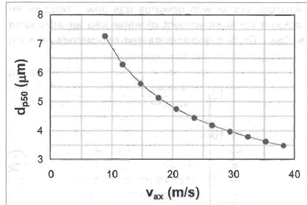
Figure 8: Axial cyclone d_{p50} as a function of mean axial velocity v_{ax} . Swirl ratio S = v_t/v_{ax} = 1.2 and L/R = 5.6 .
