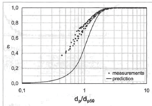
Figure 9: Measured efficiency \epsilon as a function of the particle size d_p , made non-dimensional with d_{p50} . Results below 3 \mu\text{m} were disregarded. Prediction is based on plug flow, and a Rankine vortex profile with core radius 0.8R .
