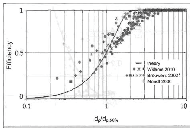
Figure 10: Efficiency of the RPS.
