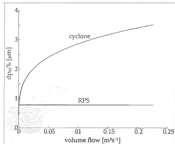
Figure 4: Diameter of water droplets in air separated by a cyclone and RPS as a function of the volume flow under atmospheric pressure.
