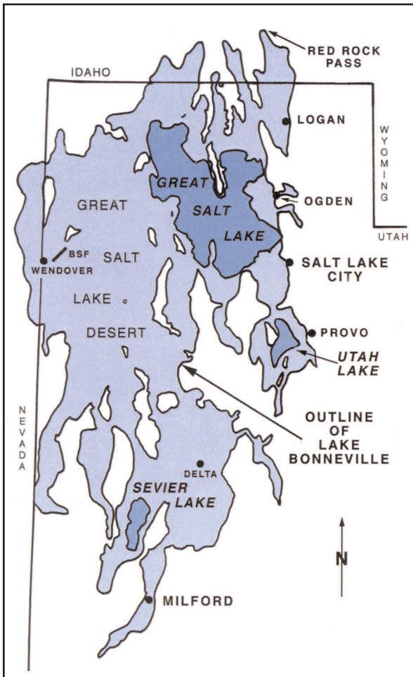
Outline of ancient Lake Bonneville and associated modern features. (BSF = Bonneville Salt Flats).
