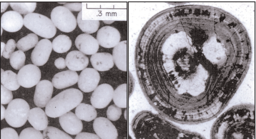
Magnified view of typical oolites (left), and oolite cross section (right) showing concentric layers built up around a central mineral fragment.
