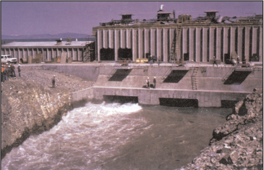
Close-up view of the pumping plant with one of the three 1,000 cubic-feet-per-second pumps in operation (view looking east).
