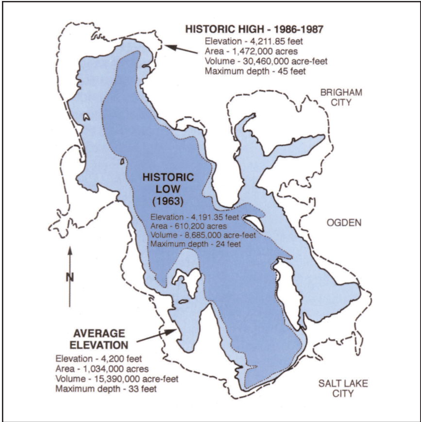
Areal extent, elevation, volume, and maximum depth of Great Salt Lake at historic high, average, and historic low-water levels.
