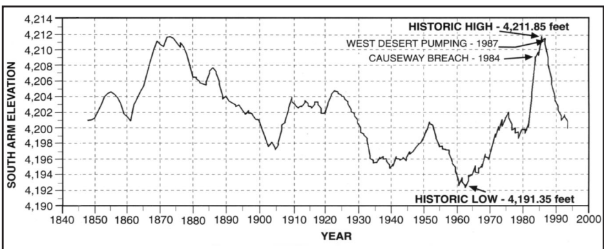
Historical elevations (in feet above mean sea level) of the surface of the southern arm of the Great Salt Lake (at its highest point for the year), 1847-1994 (USGS provisional lake records).
