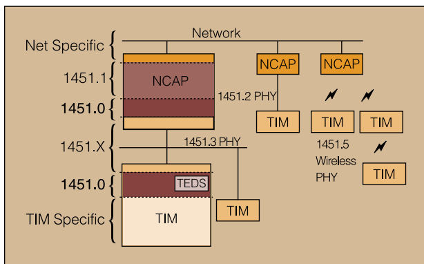
Fig. 4. Network access of IEEE 1451 wired and wireless transducers.
