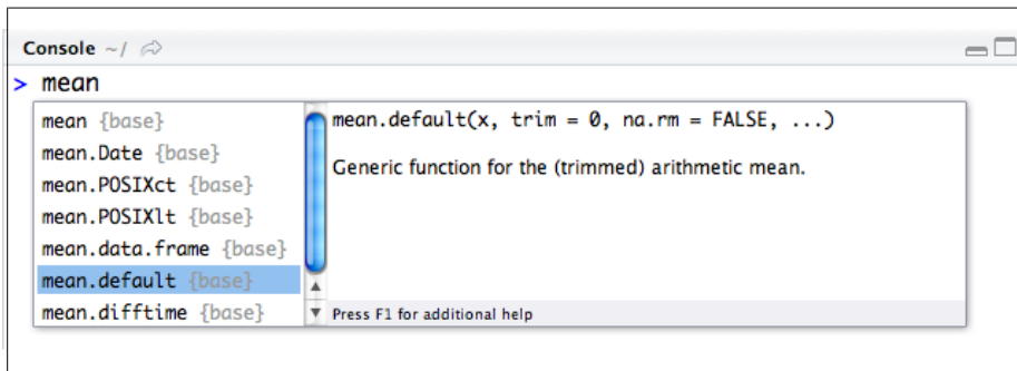
Figure 3-5. Completion for an object in the workspace shows the full name, its package (when applicable), and a short description if available
