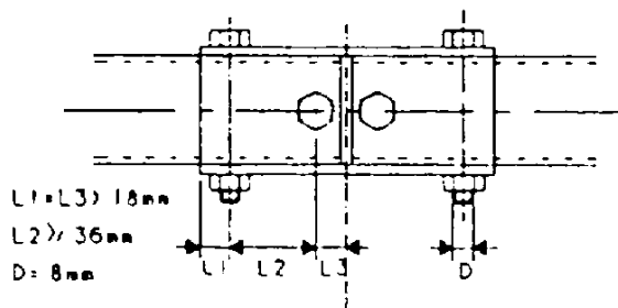
Drawing No 253-31
