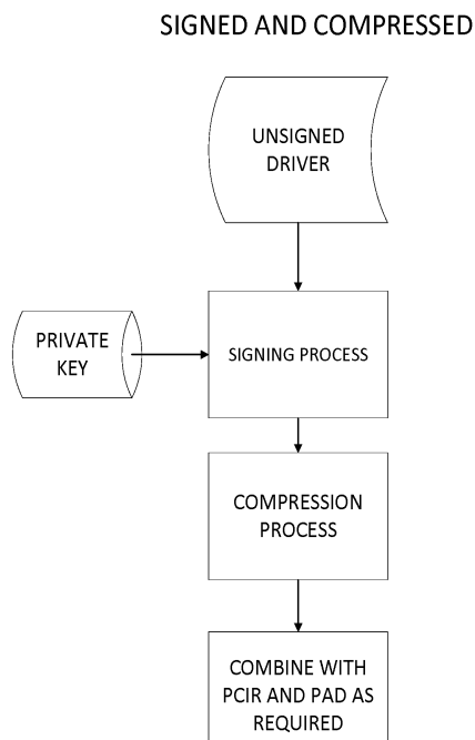
Figure 46. Signed and Compressed PCI Driver Image Flow
