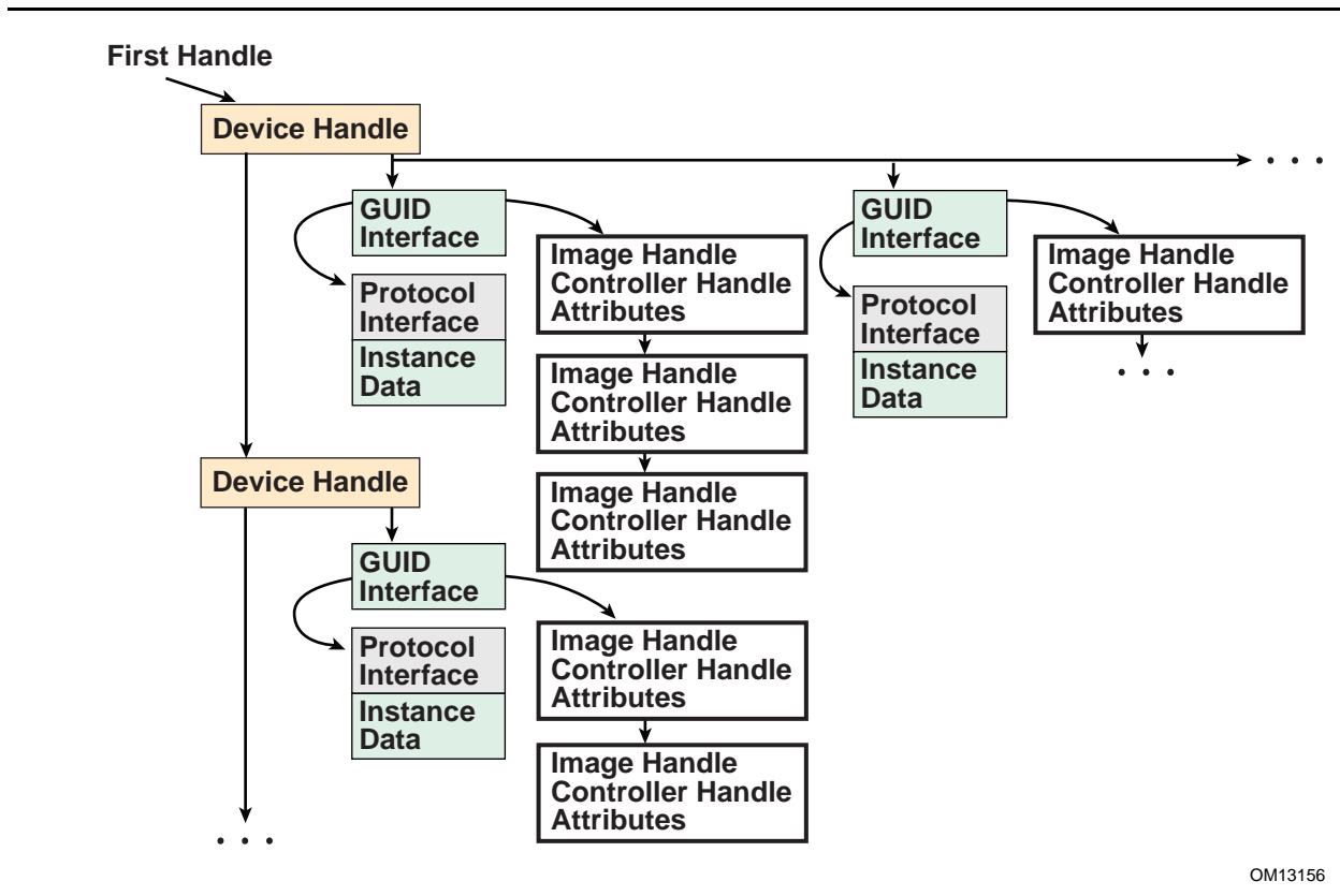
Figure 21. Handle Database
