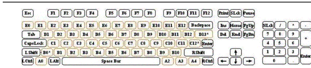
Figure 91. Keyboard Layout
