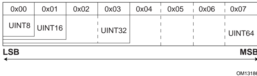
Figure 139. Storage Types
