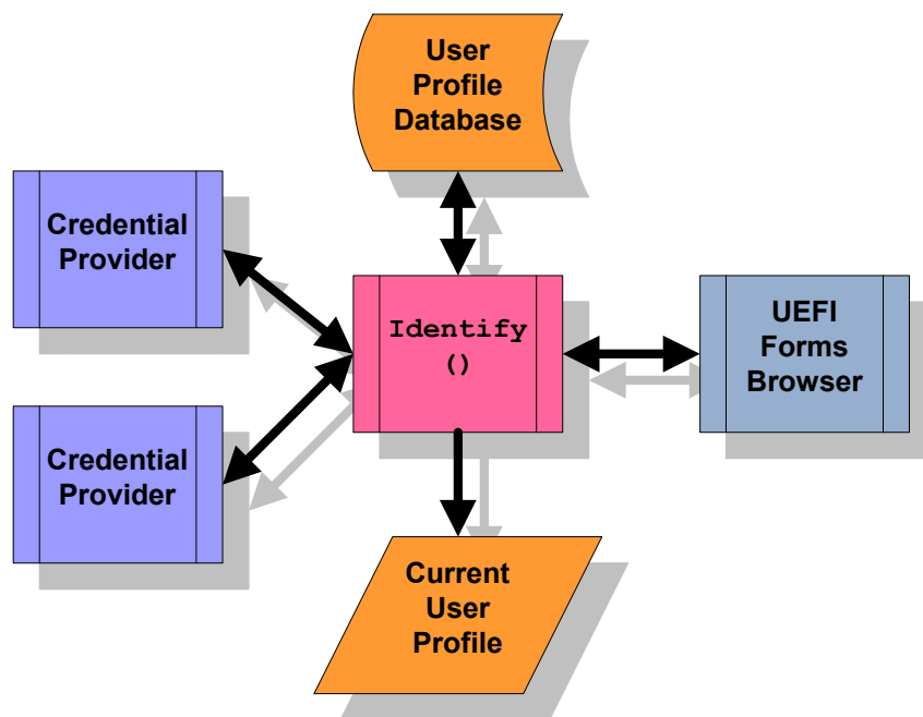
Figure 130. User Identity
