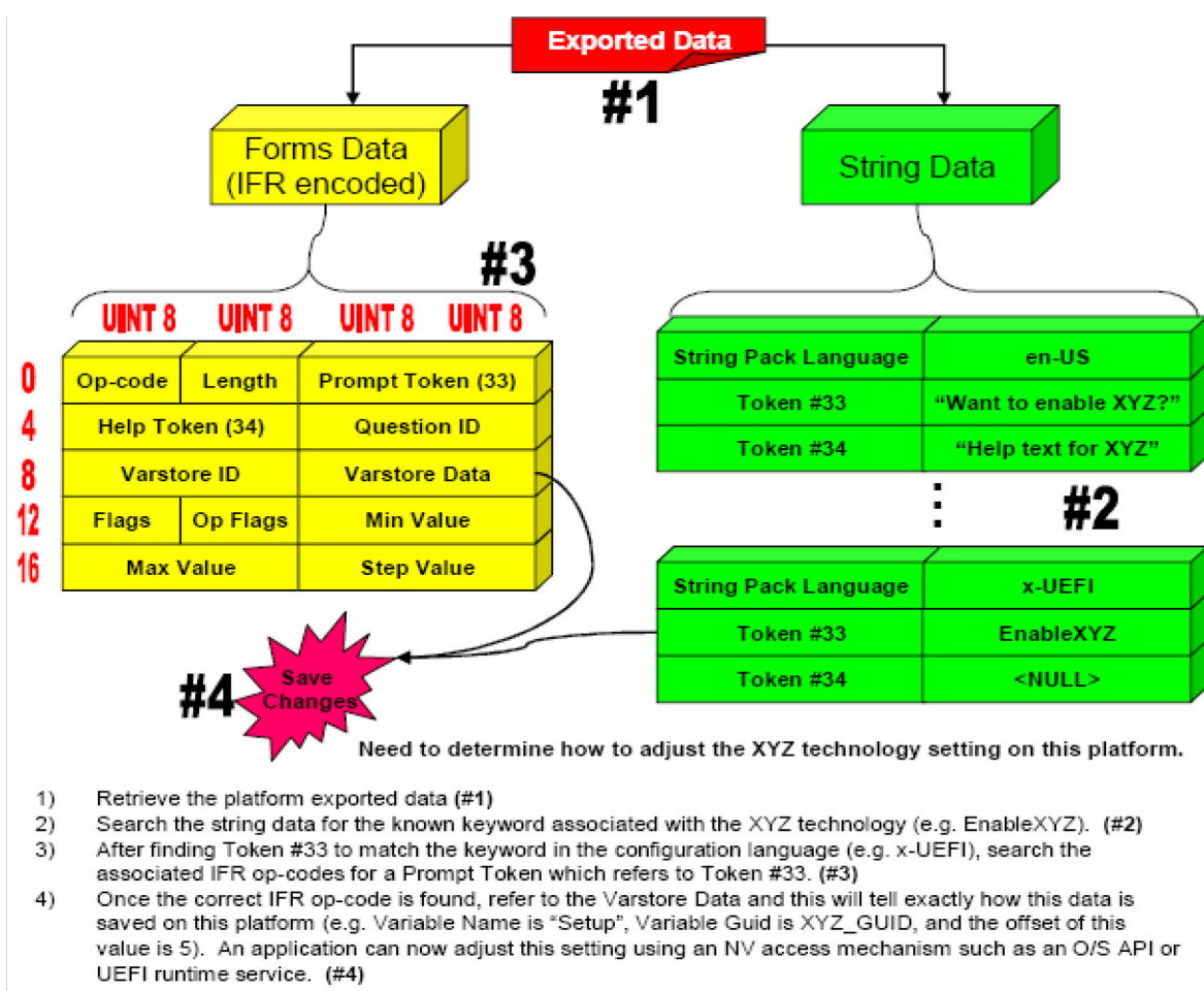
Figure 107. Standard Application Obtaining Setting Example
