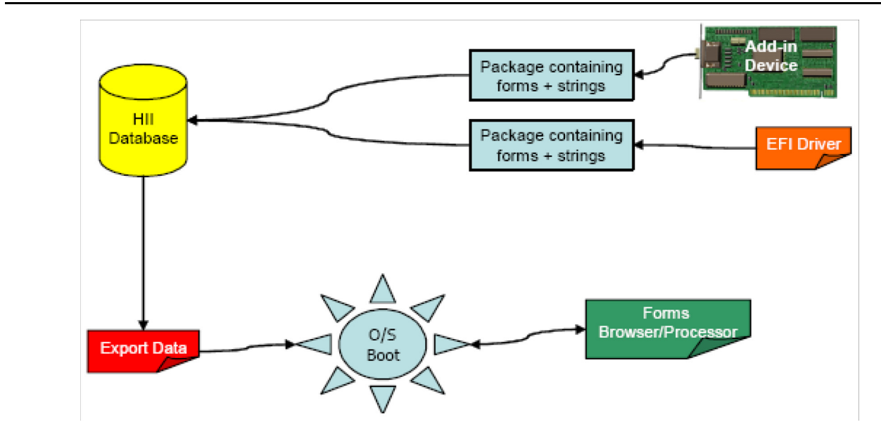
Figure 89. O/S-Present Forms Browser/Processor
