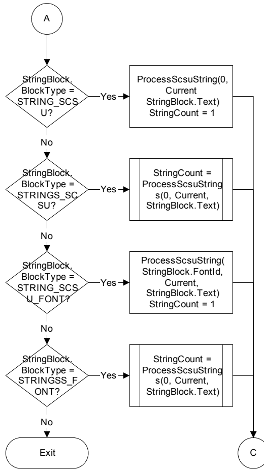
Figure 119. String Block Processing: SCSU Processing
