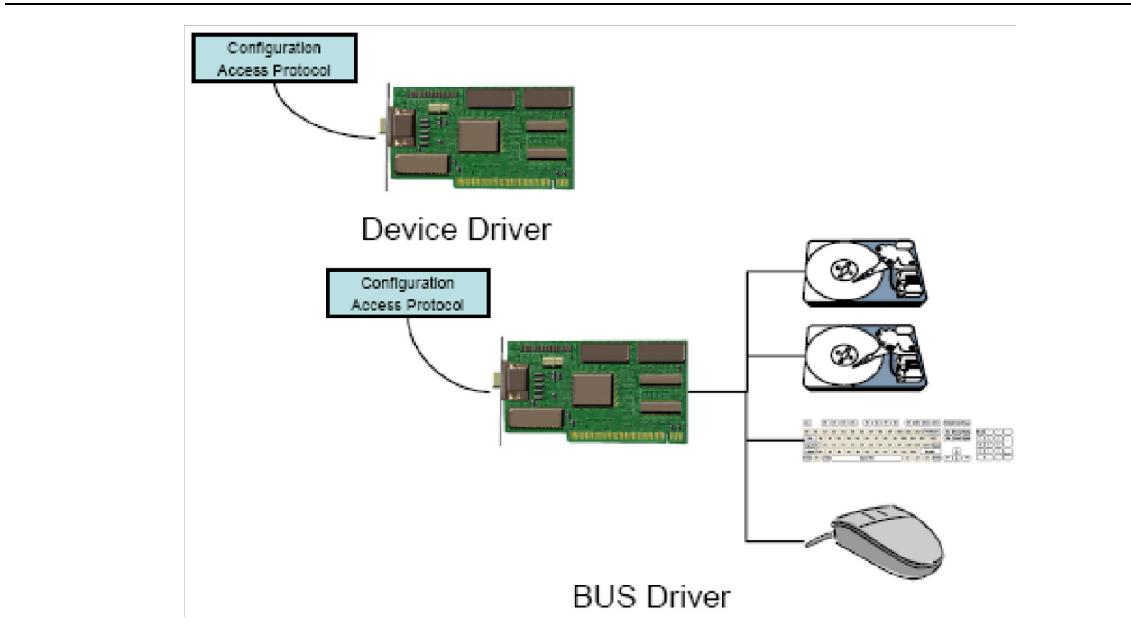
Figure 111. Driver Model Interactions
