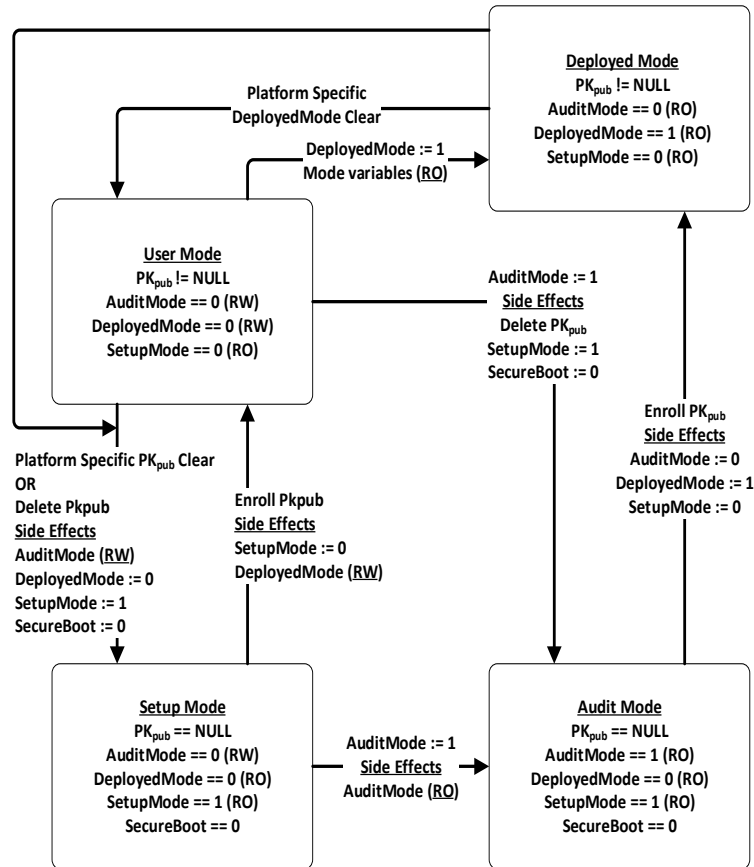
Figure 77. Secure Boot Modes
