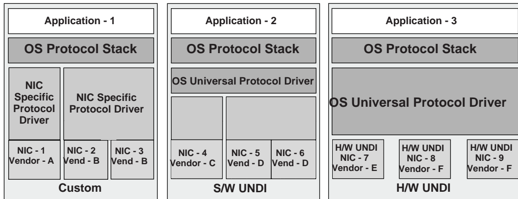
Figure 135. Network Stacks with Three Classes of Drivers
