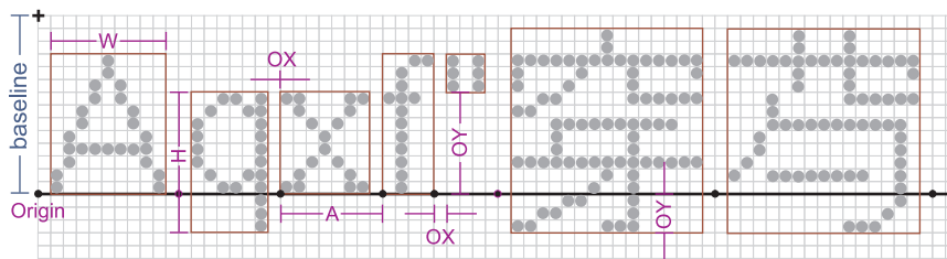
Figure 102. Aligning Glyphs
