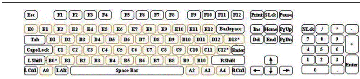
Figure 129. Keyboard Layout
