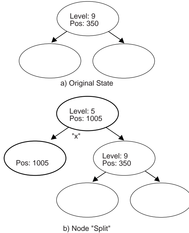
Figure 61. Node Split
