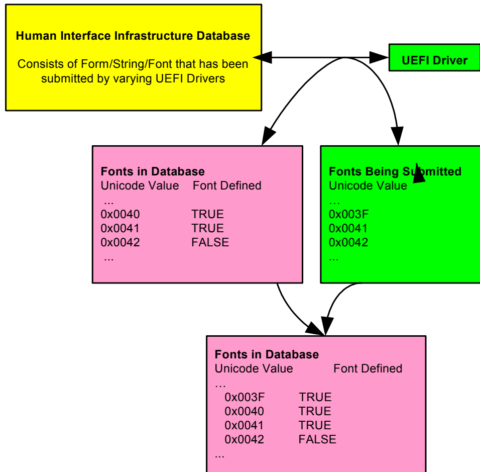
Figure 97. Fonts
