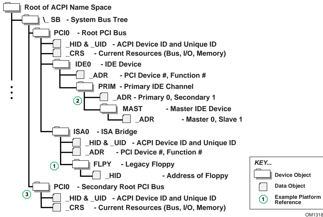
Figure 133. Partial ACPI Name Space for Example System
