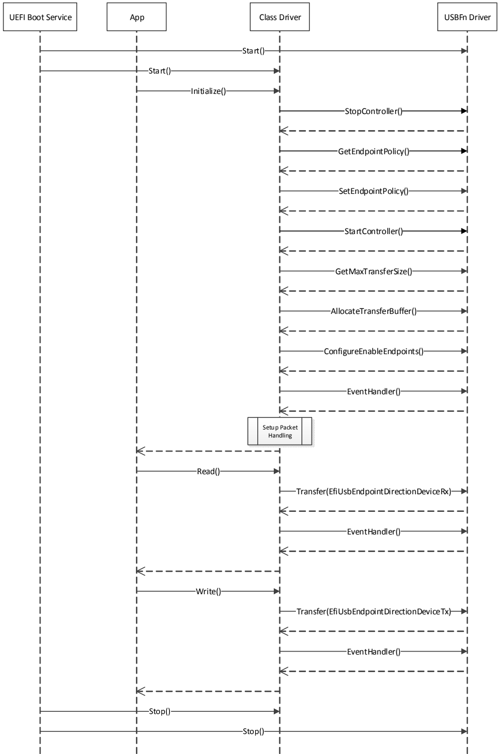
Figure 54. Sequence of Operations with Endpoint Policy Changes
