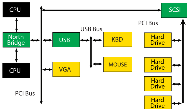
Figure 7. Server System
