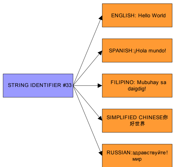
Figure 96. String Identifiers
