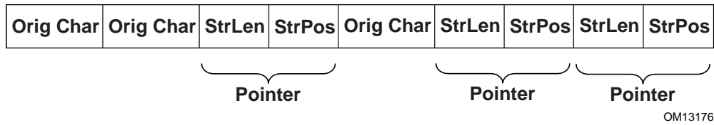
Figure 59. Block Body
