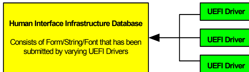
Figure 103. HII Database
