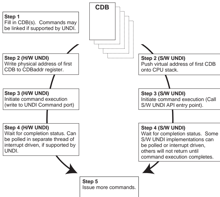
Figure 137. Issuing UNDI Commands
