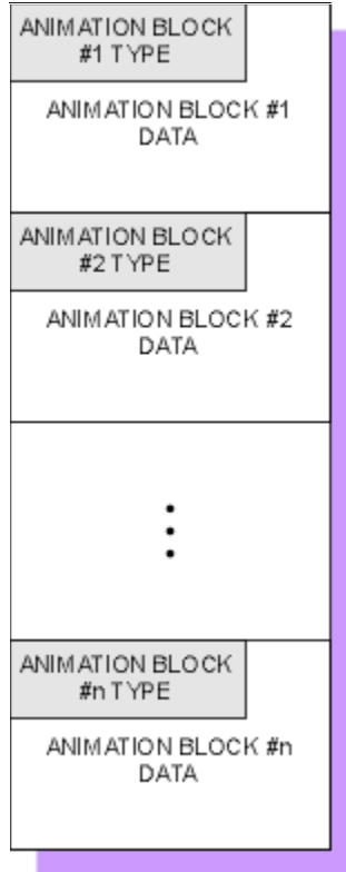
Figure 128. Animation Information Encoded in Blocks
