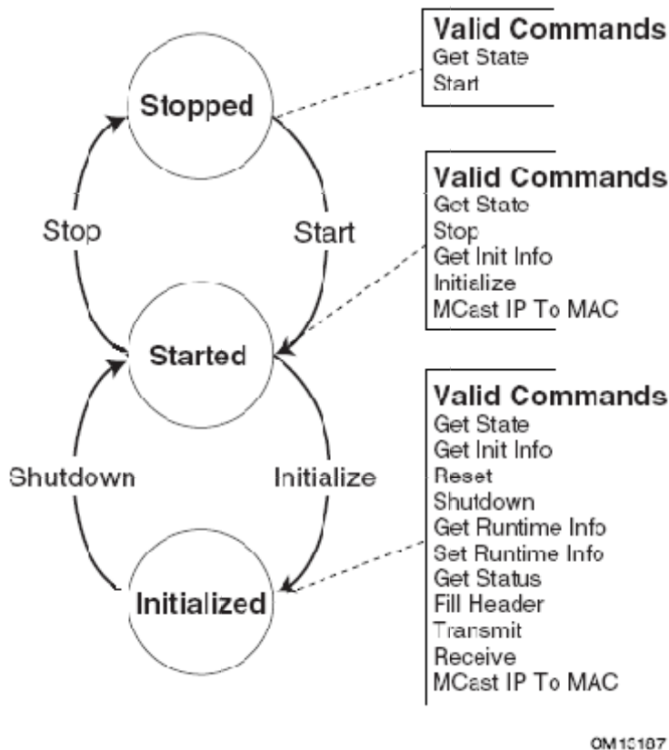
Figure 140. UNDI States, Transitions & Valid Commands
