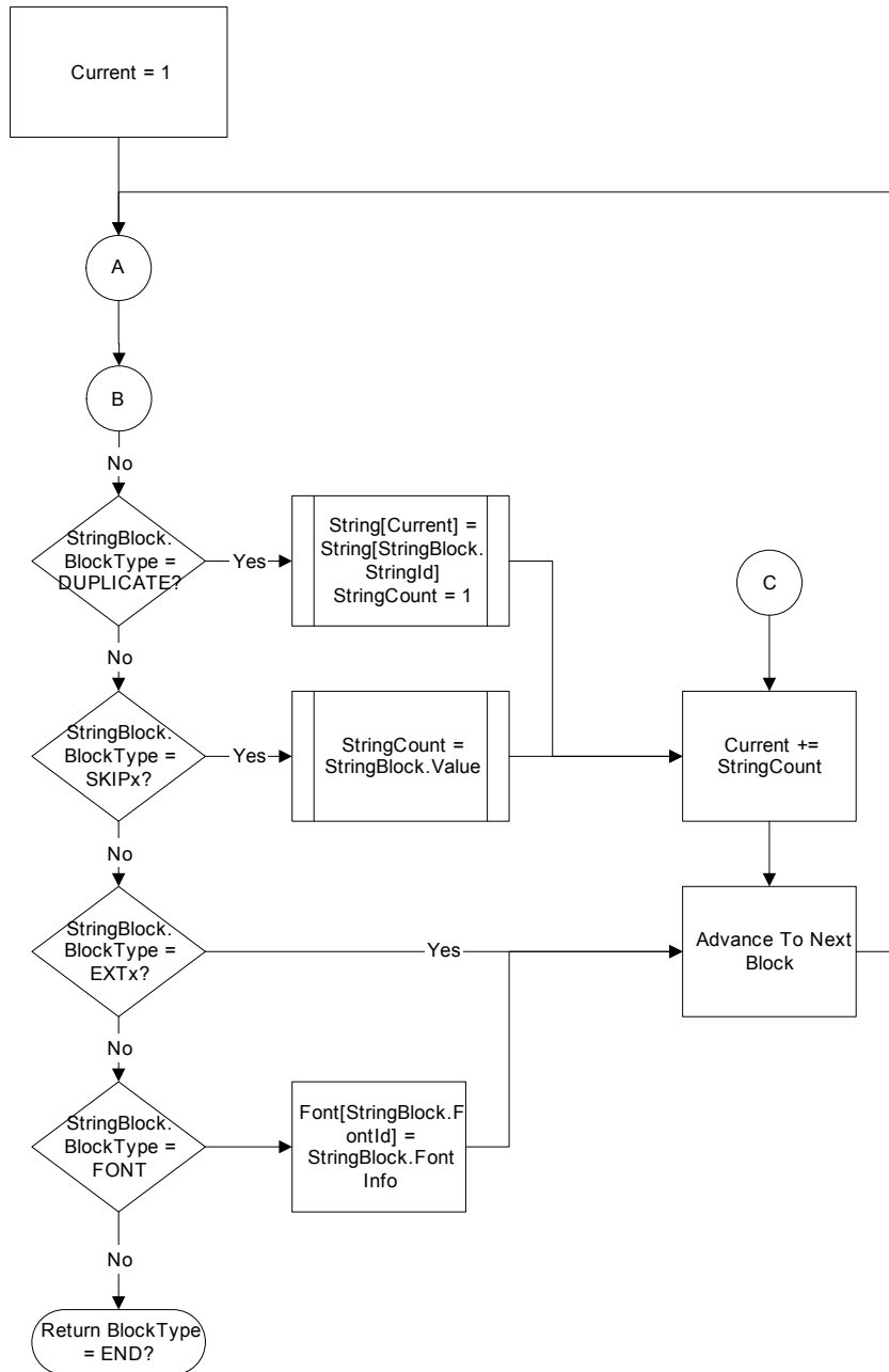
Figure 118. String Block Processing: Base Processing
