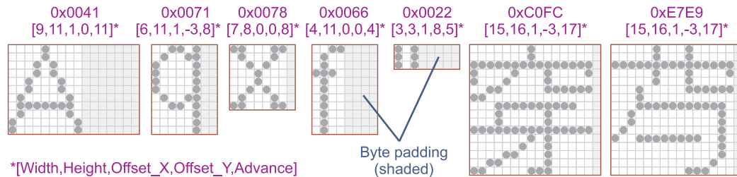
Figure 101. Proportional Font Parameters and Byte Padding
