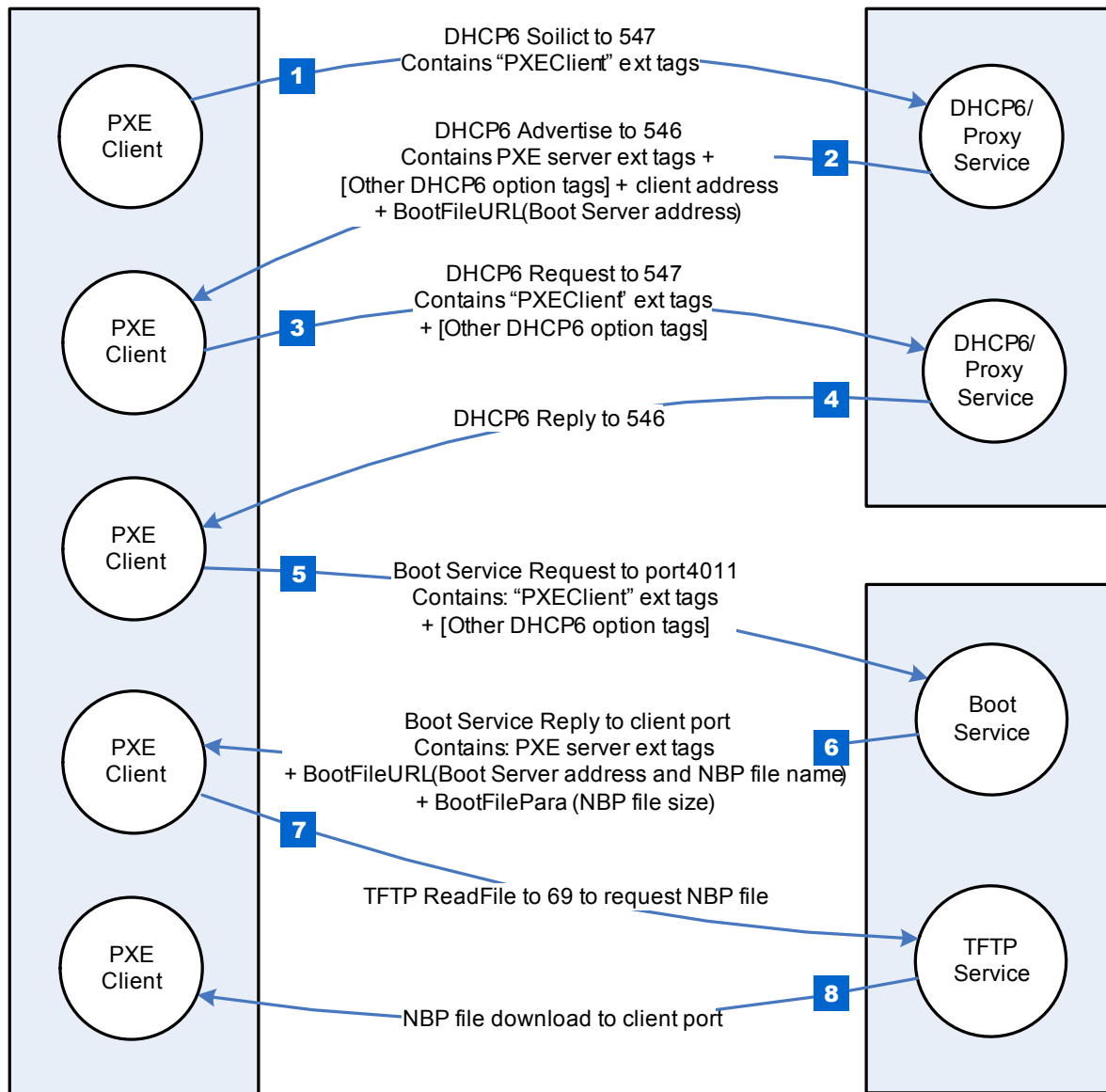
Figure 67. IPv6-based PXE boot
