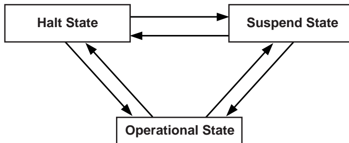
Figure 52. Software Triggered State Transitions of a USB Host Controller
