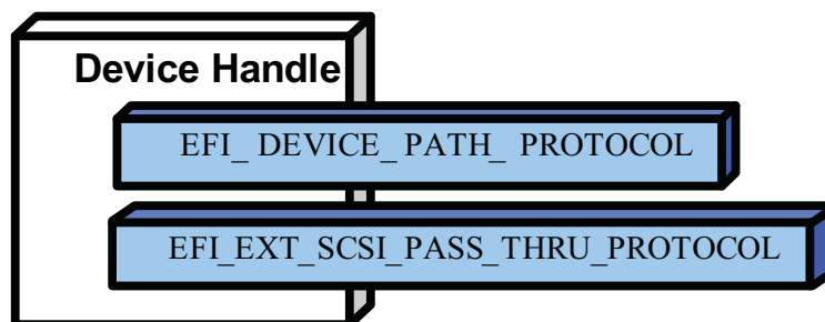
Figure 50. Device Handle for a SCSI Bus Controller
