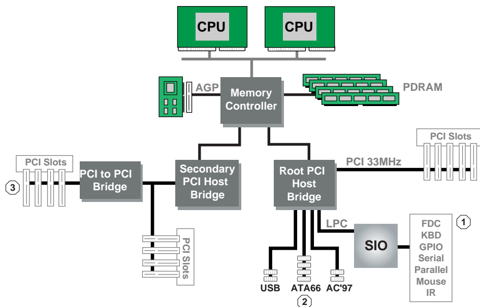
Figure 132. Example Computer System
