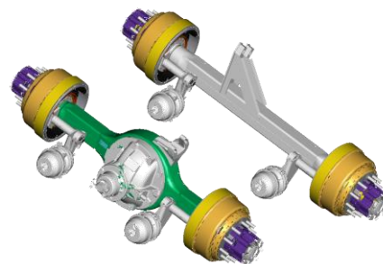
“Tag Tandem” – One Driving Axle
