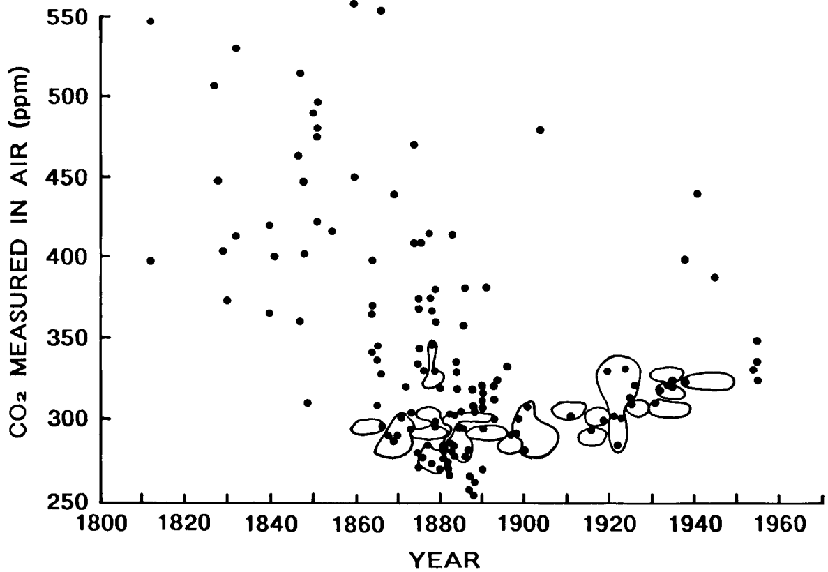
Figure 4. Average atmospheric CO 2 concentrations measured in the 19th and 20th century. Encircled are the values used by Callendar (1958). Redrawn after Fonselius et al. (1956).
