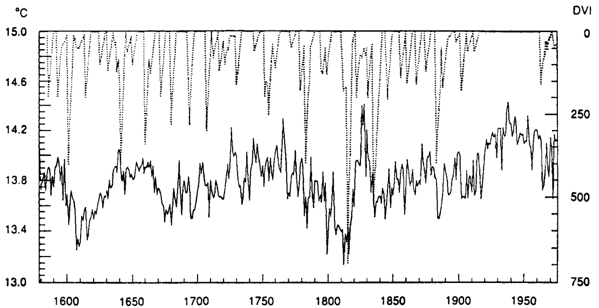
Figure 9. Lower curve: Northern Hemisphere annual temperatures (data from Borzenkova et al., 1976 and Groveman and Landsberg, 1979). Upper curve: Volcanic Dust Veil Index, D.V.I. (data from Lamb 1970, 1978), with increasing values downwards.
