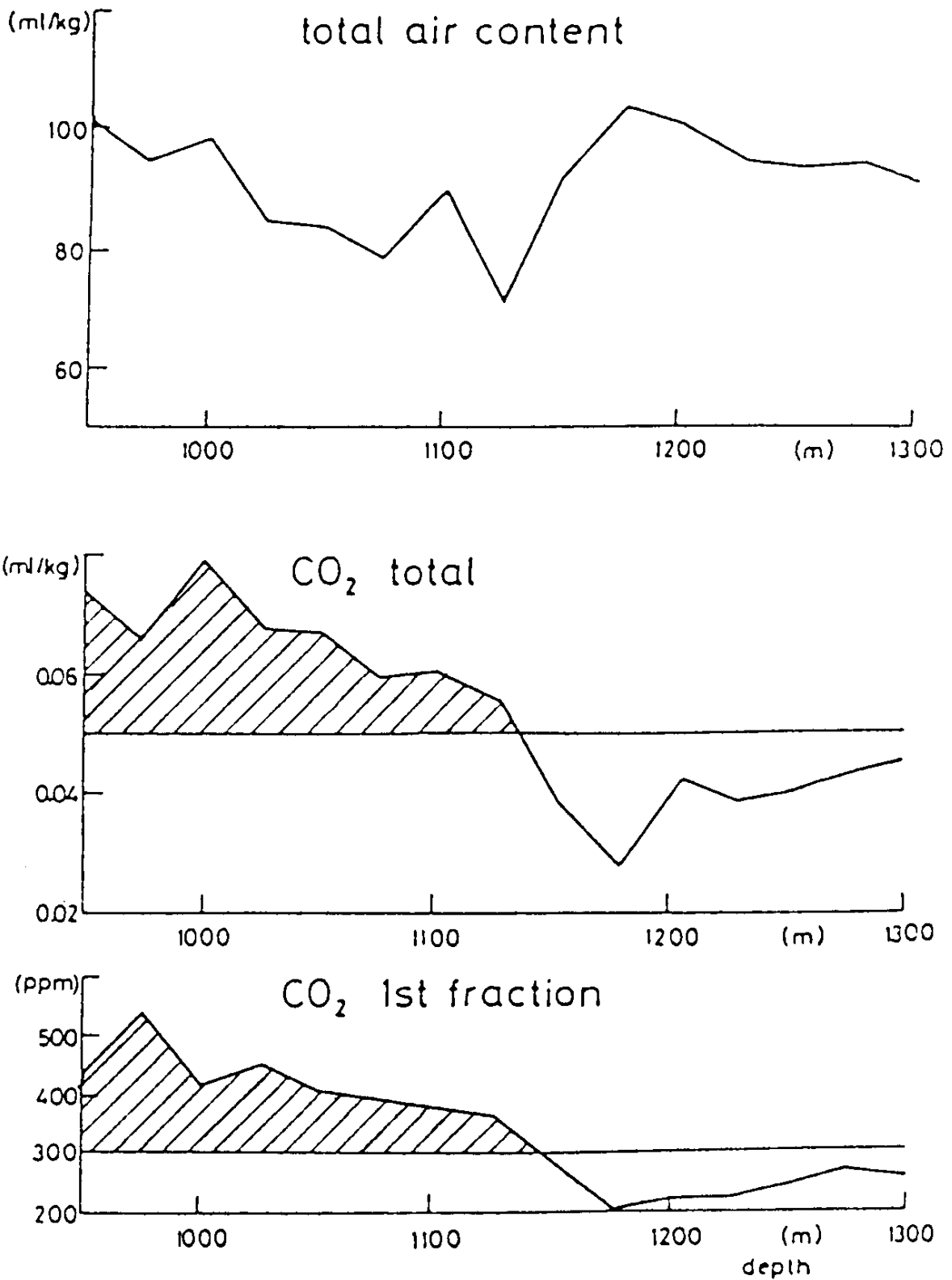
Figure 5. Changes of air and CO 2 content in glacier ice from Camp Century (Greenland) versus depth (after Berner et al., 1980). Note the decrease in CO 2 content below ~1130 m, where air bubbles were reported to disappear.
