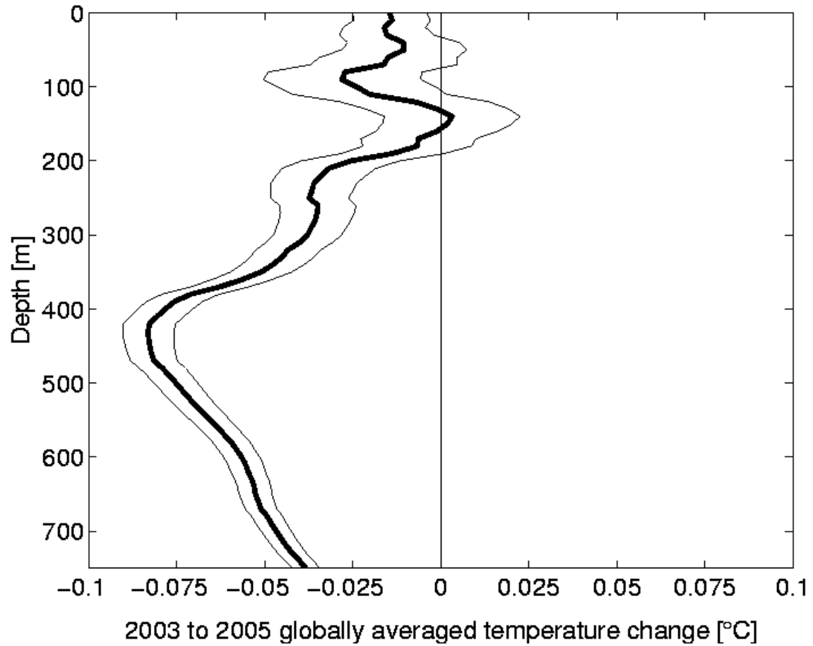
Figure 4. Globally averaged ocean temperature change [°C] from 2003 to 2005 versus depth [m]. Thin black lines represent error bounds determined by scaling the uncertainty in heat content using regression coefficients [Willis et al. , 2004].
