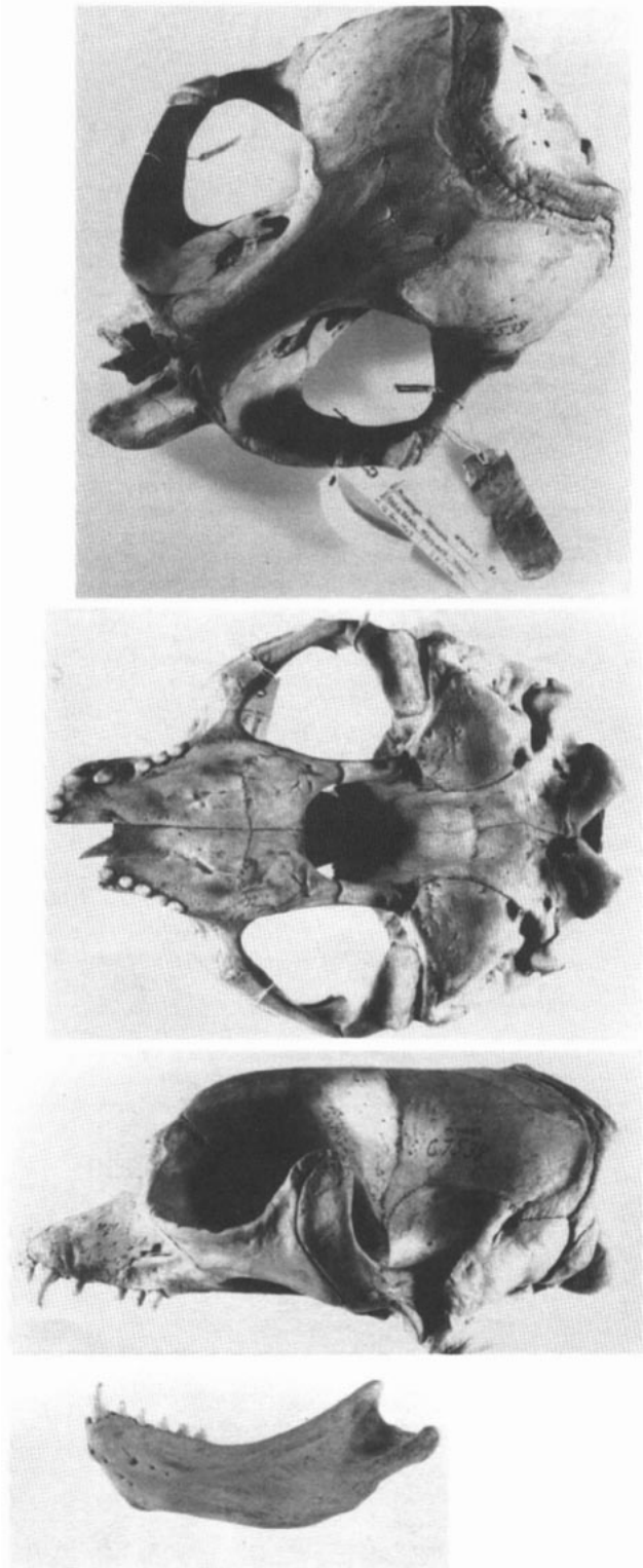
FIG. 3. Dorsal, ventral, and lateral views of cranium and lateral view of mandible of female Mirounga leonina (South Australian Museum M14447 from Macquarie Island). Condylbasal length of cranium is 285.0 mm.
