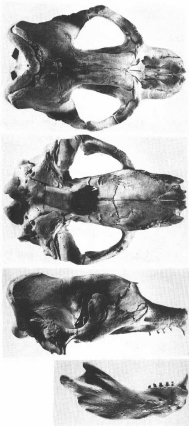
FIG. 2. Dorsal, ventral, and lateral views of cranium and lateral view of mandible of a male Mirounga leonina (South Australian Museum M3744 from Adelie Land, Antarctica). Condylbasal length of cranium is 324.0 mm.
