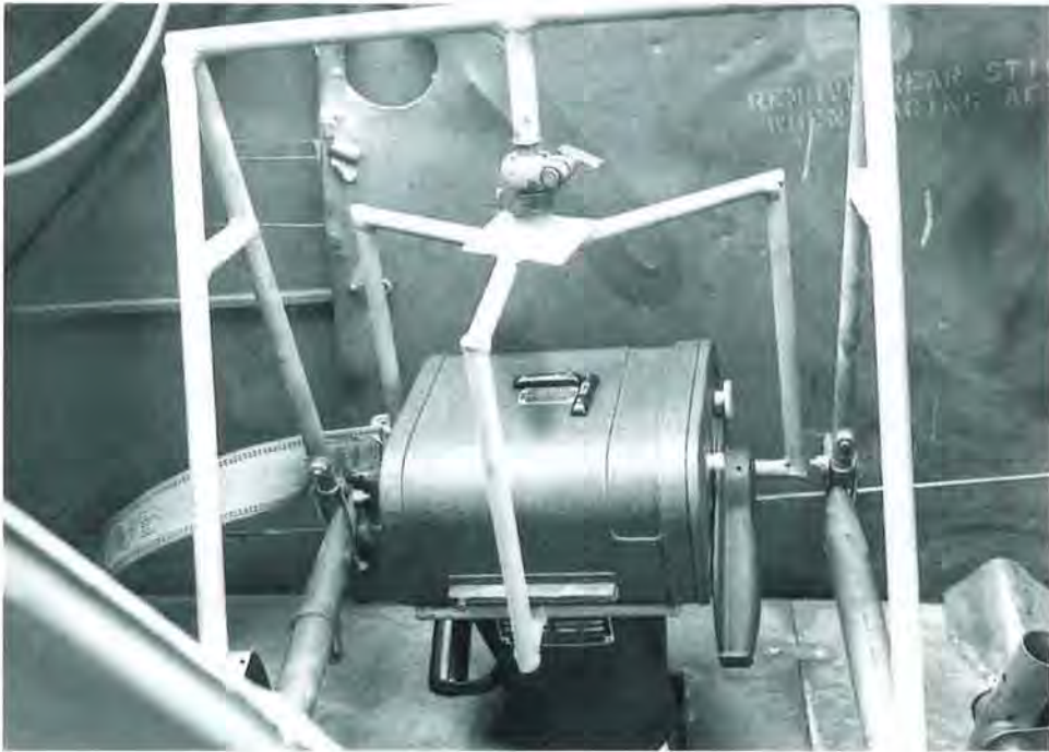
A K-20 AERIAL CAMERA IN A SPECIAL MOUNT ON AN L-4H, ALLOWING THE CAMERA TO TAKE VERTICAL PHOTOGRAPHS
