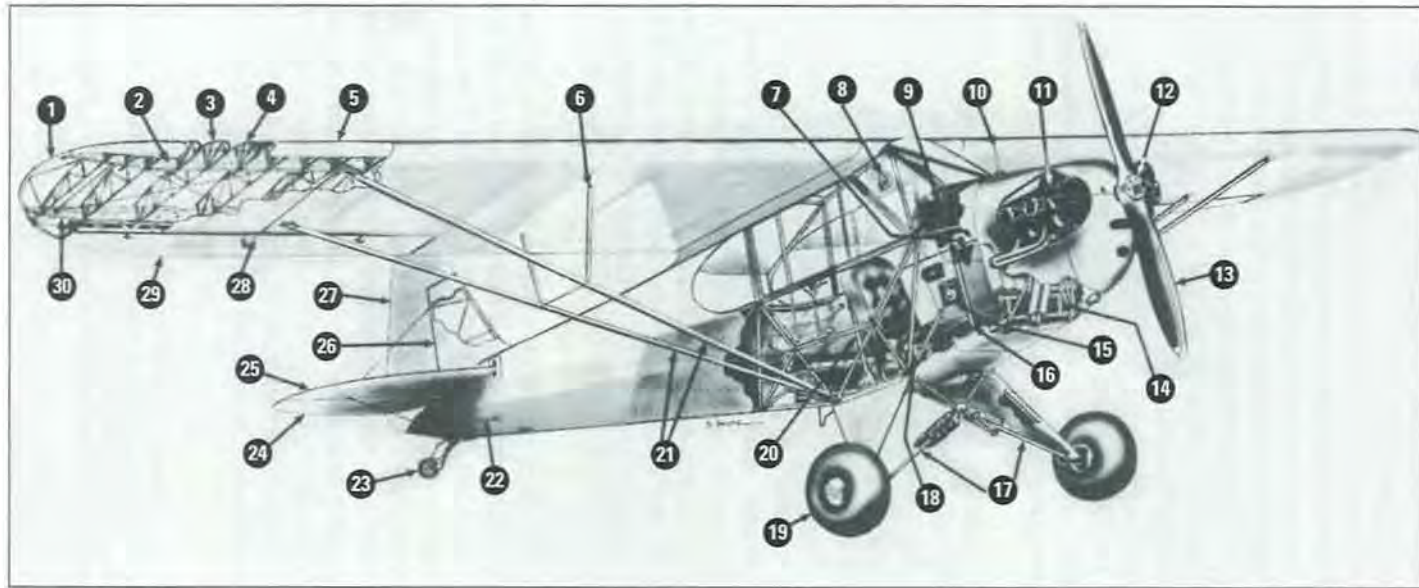
FIGURE 1—CROSS-SECTIONAL DIAGRAM OF A PIPER CUB
