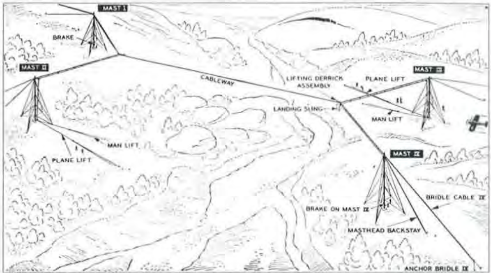
FIGURE 4—LAND INSTALLATION OF THE BRODIE DEVICE
