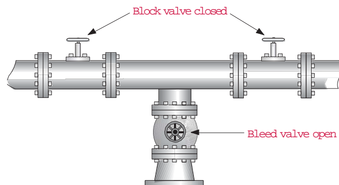
Double block and bleed
