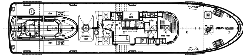
FORECASTLE DECK
