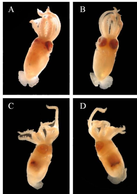
Figure 5.31. Histioteuthis sp.: dorsal (A) and ventral (B) views, 1.6 mm ML; lateral (C) and dorso-lateral (D) views, 3.6 mm ML.
