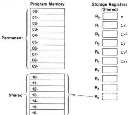
Program Memory Allocation:
