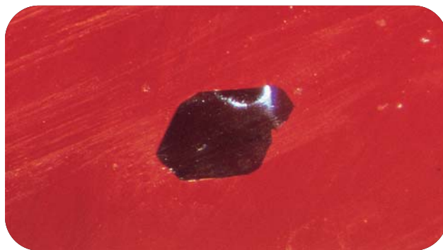
Figure 12. This opaque black inclusion was identified as hematite by Raman analysis. Photomicrograph by James Shigley; magnified 15 \times .
