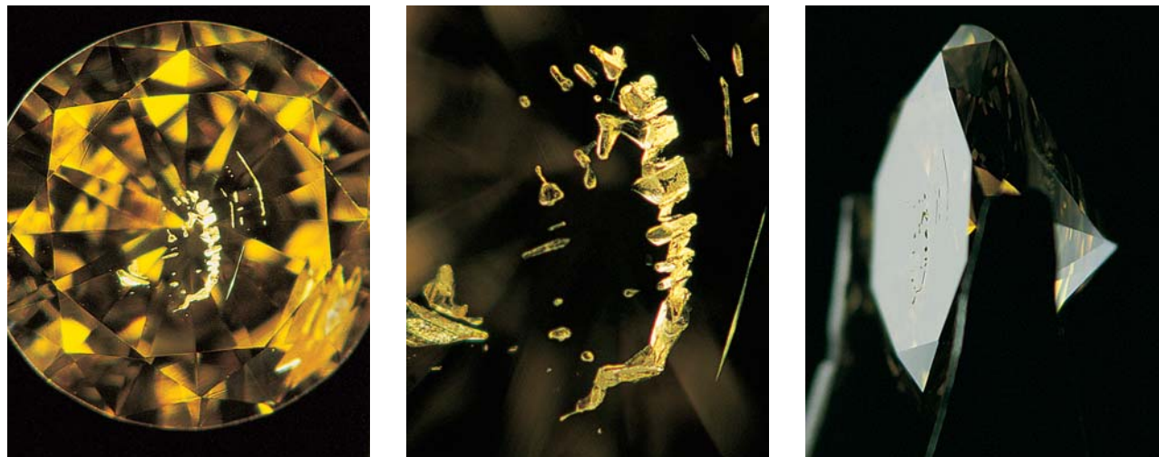
Figure 13. Left: Large cavities were visible on the table of this 0.52 ct orangy yellow synthetic diamond at relatively low magnification (15×). Center: At higher magnification (45×), it is evident that these cavities are amorphous rather than crystalline in shape. Right: Examination with reflected light confirmed that the cavities were not related to surface-reaching inclusions but were probably the result of flux inclusions that had been dissolved during an acid cleaning after polishing (magnified 15×).
