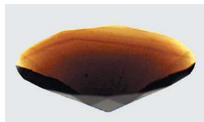
Figure 2. Immersion in methylene iodide made it easy to distinguish between the yellow bodycolor of the 5.73 ct andradite and its straight, angular, red-brown color banding.
