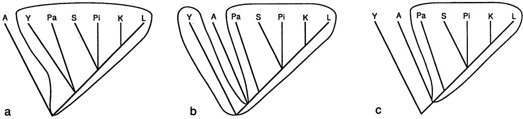
FIG. 2. Phylogenetic definitions and monophyly. (a) Phylogenetic relationships within Sauria, with bubble encircling Lepidosauromorpha as its name was defined by Gauthier et al. (1988a). (b) Hypothetical change in ideas about the relationships of Younginiformes (Y), which seems to imply paraphyly of Lepidosauromorpha when the content rather than the definition is considered. (c) The actual limits and monophyly of Lepidosauromorpha under the revised relationships according to the definition as stated. See text for additional discussion. Abbreviations: A, Archosauria; Y, Younginiformes; Pa, Palaeagama *; S, Saurosternon *; Pi, Paliguana *; K, Kuehneosauridae; L, Lepidosauria.
