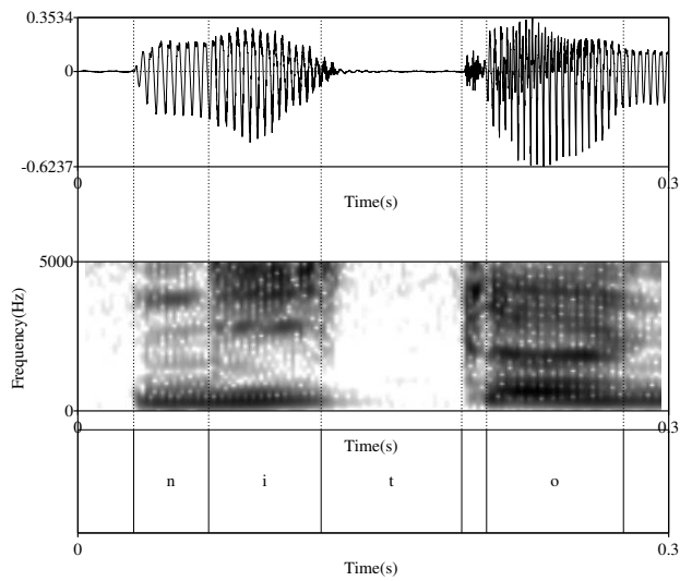
Figure 1: A singleton [t] in Japanese. The time scale is 300ms.
