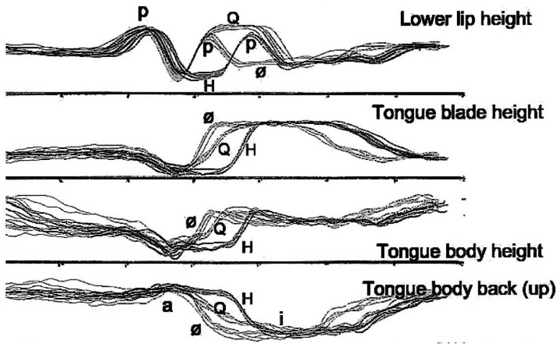
Figure 6: The articulatory movements of Japanese geminates, as compared to singletons. Based on Ishii (1999), cited and discussed in Fujimura & Williams (2008). Three conditions are [papa] ( \phi ), [paapa] (H), and [pappa] (Q).
