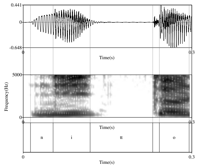
Figure 2: A geminate [tt]. The time scale is 300ms.
