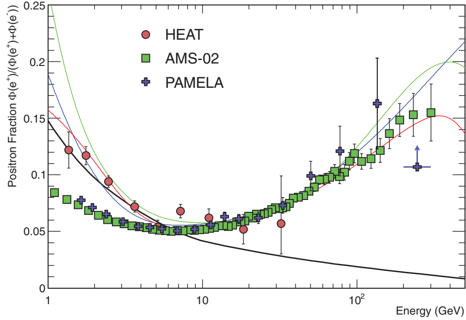
Figure 28.3: The positron fraction (ratio of the flux of e^+ to the total flux of e^+ and e^- ) [24,25,28]. The heavy black line is a model of pure secondary production [26] and the three thin lines show three representative attempts to model the positron excess with different phenomena: green: dark matter decay [27]; blue: propagation physics [30]; red: production in pulsars [38]. The ratio below 10 GeV is dependent on the polarity of the solar magnetic field.
