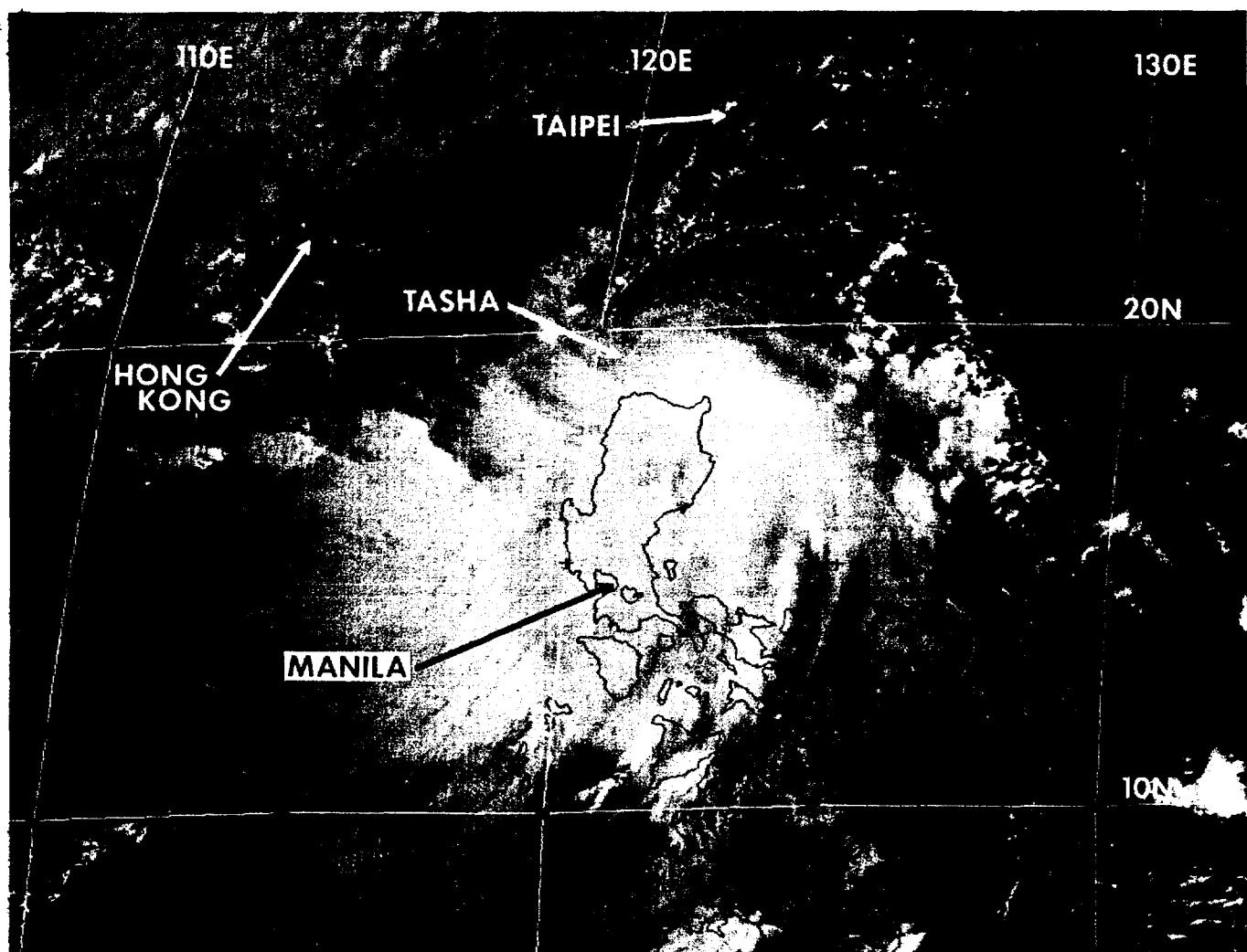
Figure 3-16-1 As Tasha passes north of Manila, bands of deep convection cover the island of Luzon (172331Z August visual GMS imagery.)
