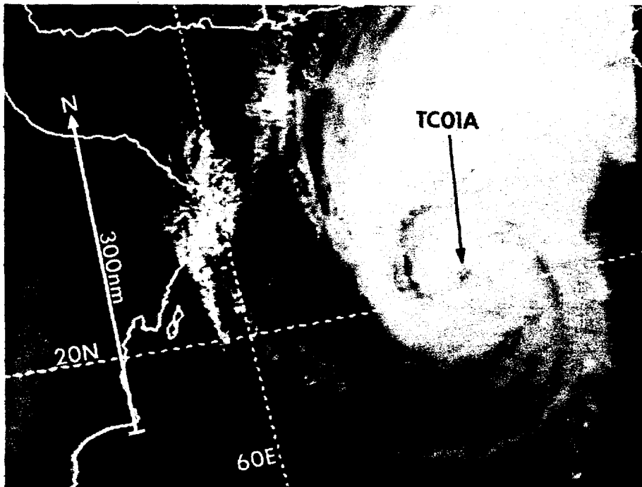
Figure 3-01A-1 TC 01A in the central Arabian Sea is within 12 hours of reaching its peak intensity of 80 kt (41 m/sec) (140059Z November visible DMSP image).
