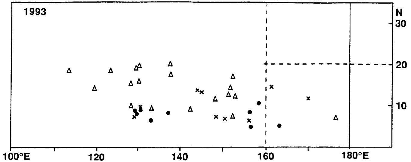
Figure 3-5a Point of formation of significant tropical cyclones in 1993 as indicated by the initial intensity of 25 kt (13 m/sec) on the best track. The symbols indicate: solid dots = 01 January to 15 July; open triangles = 16 July to 15 October; and, X = 16 October to 31 December.
