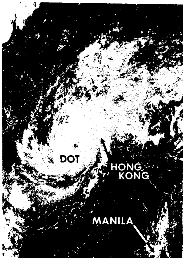
Figure 3-24-1 The eye of Dot, which is located southwest of Hong Kong, is visible in the moonlight. The city lights of Hanoi and Manila can also be seen (251321Z September nighttime visual DMSPI imagery).
