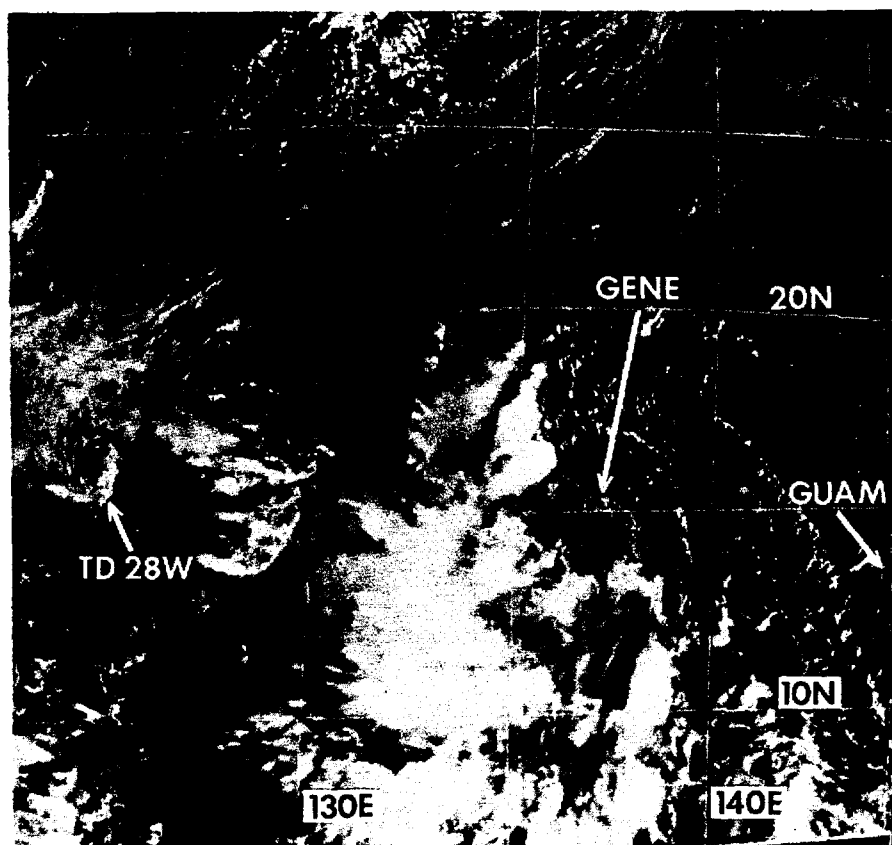
Figure 3-27-1 Cloud lines outline the exposed low-level circulation center of Gene about 12 hours before it was upgraded to tropical storm intensity (080424Z October visible DMSPP imagery).
