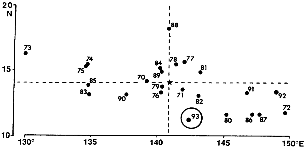
Figure 3-5b Mean annual genesis locations for the period 1970-1993. The 1993's circled location is the southernmost for the 24 years. The star lies at the intersection of the 24-year average latitude and longitude of genesis. For statistical purposes, genesis is defined as the first 25 kt (13 m/sec) intensity on the best track.
