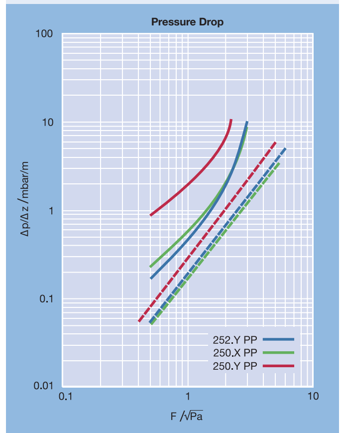
Mellapak PP atmospheric pressure
