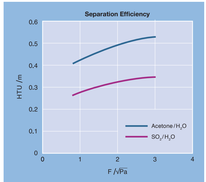
Separation efficiency of Mellapak 250.Y PP
