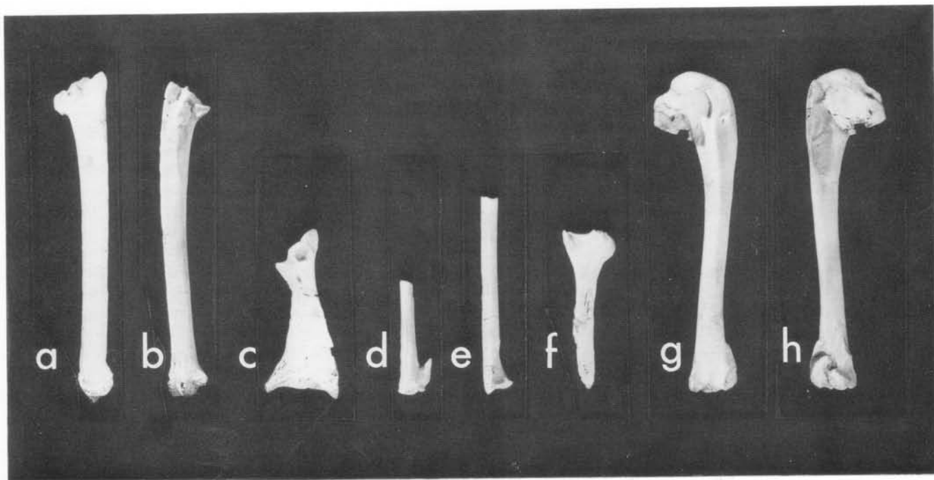
Figure 2. Uria paleohesperis n. sp. and Cepphus olsoni n. sp., natural size Parts a through f , U. paleohesperis n. sp., holotype, UCMP 88704. Parts a and b , left ulna, external and internal views. Part c , right coracoid, dorsal (posterior) view. Part d , distal end of left carpometacarpus, external view. Part e , distal end of right radius, palmar view. Part f , right scapula, dorsal view. Parts g and h , C. olsoni , n. sp., holotype, LACM 107032, humerus, anconal and palmar views.
