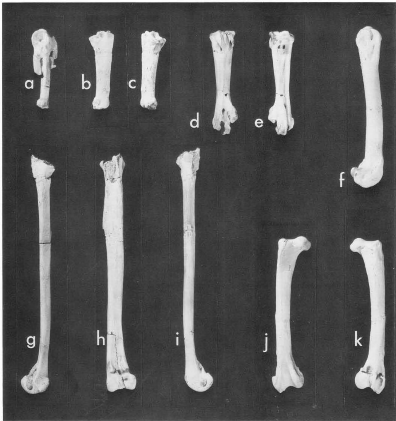
Figure 3. Praemancalla cf. P. wetmorei , natural size, a–e and g–i, LACM 107028, f, j, k, SDSNH 21101. Part a , carpometacarpus, internal view. Parts b and c , ulna, external and internal views. Parts d and e , tarsometatarsus, posterior and anterior views. Parts f, j, and k , femur, external, anterior, and posterior views. Parts g, h, and i , tibiotarsus, internal, anterior, and external views.
