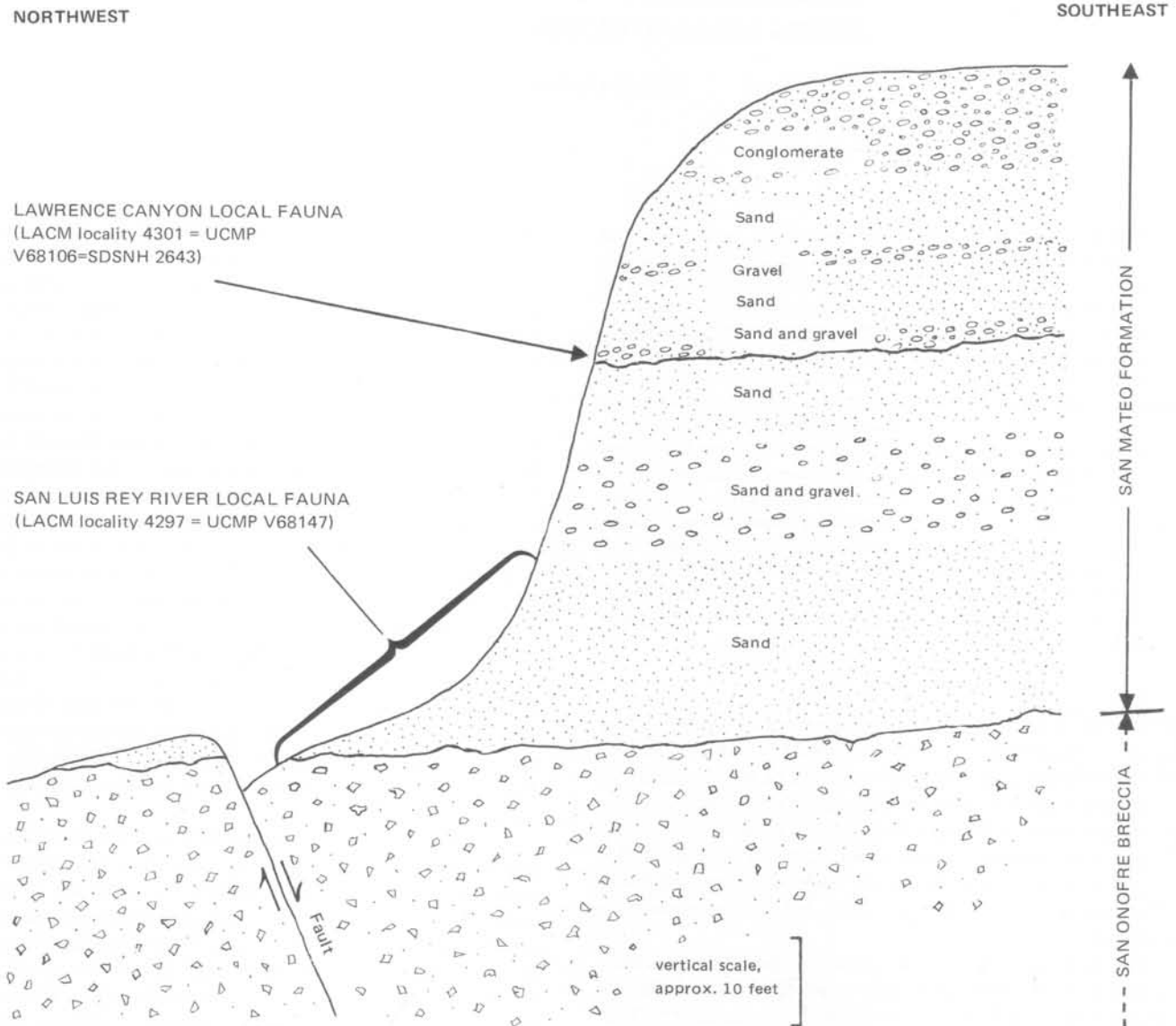
Figure 1. Diagrammatic geologic cross section of part of the San Mateo Formation and the San Onofre Breccia exposed in Lawrence Canyon at Oceanside, showing the stratigraphic occurrence of some fossils making up the two local faunas. Relative thicknesses of the beds are estimated, and the amount of displacement on the fault has not been measured. There is an unconformity at the contact between the San Mateo Formation and the San Onofre Breccia, and another within the San Mateo Formation at the base of the sand and gravel bed that produced the Lawrence Canyon Local Fauna. The San Luis Rey River Local Fauna is derived from the entire thickness of the lowest sand unit resting unconformably upon the San Onofre Breccia. Modified from Barnes et al, 1981, fig. 1. Based on notes and sketches made in the field by Barnes.
