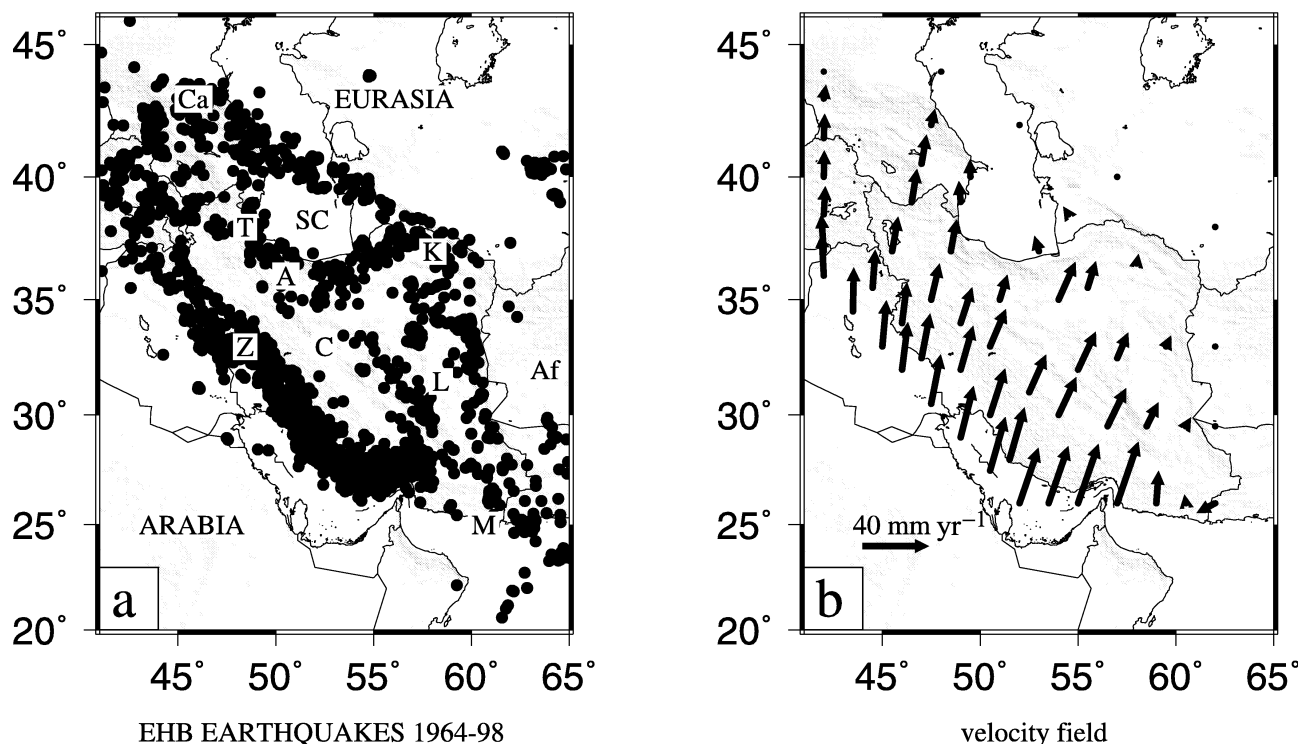
Figure 1. (a) Seismicity of Iran 1964–98, with epicentres from the catalogue of Engdahl et al. (1998). The Zagros is marked by Z, the Alborz by A, the Koppeh Dagh by K, the Talesh by T, the South Caspian Basin by SC, the Caucasus by Ca, Afghanistan by Af, the Makran by M, the relatively aseismic central Iran block by C, and the Lut block by L. (b) A velocity field showing how the northward motion of Arabia relative to Asia is absorbed in Iran. The distribution of velocities within Iran is estimated from the spatial variation in the style of strain rates indicated by earthquakes (from Jackson et al. 1995). The velocity of the Arabian margin (SW border of Iran) was based on the Arabia–Africa motion estimated by Jestin et al. (1994), and probably has too great an eastward component. Recent GPS-based estimates of Arabia–Eurasia motion are slower, and suggest a more N–S direction of convergence (Tatar 2001; Hessami 2002; Sella et al. 2002), closer in direction to that predicted by De Mets et al. (1994); see Fig. 2.
