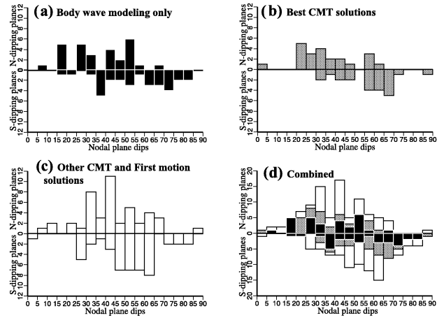
Figure 11. Histograms of nodal plane dips for reverse and thrust faulting earthquakes (with rake in the range 60–120°). Both nodal planes are included for each earthquake. (a) Earthquakes whose mechanisms are determined by P and SH body wave modelling, and N- or NE-dipping planes are distinguished from those dipping S or SW. (b) The ‘best’ CMT solutions, with M_w \geq 5.3 and >70 per cent double-couple component. (c) Other CMT solutions. (d) All earthquakes in (a)–(c) combined.
