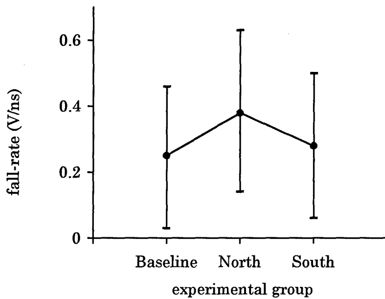
Figure 4-10. Fall-rate with a magnet in the cathode.
