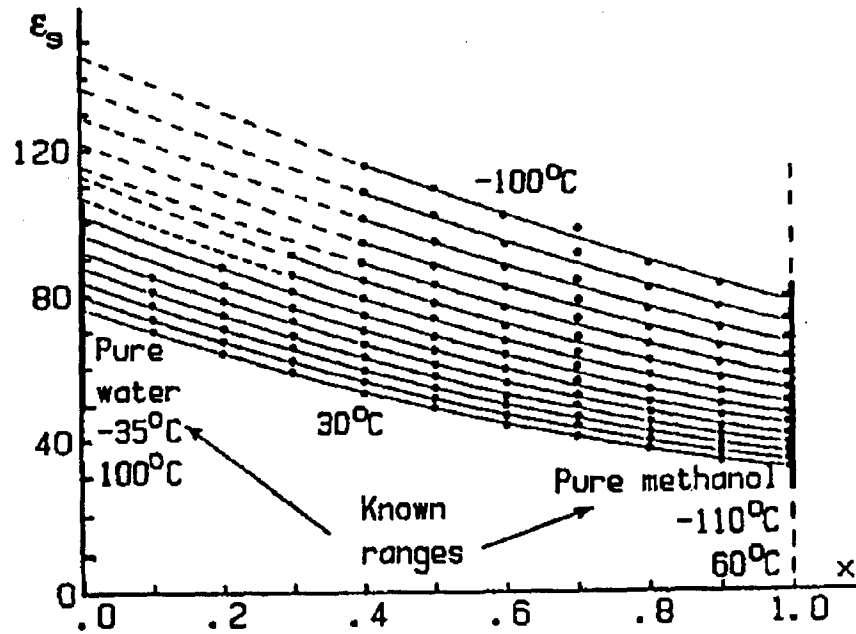
Figure 2-2. Isothermal static permittivity versus molar fraction x for mixtures (\text{methanol})_x / (\text{water})_{1-x} [5].
