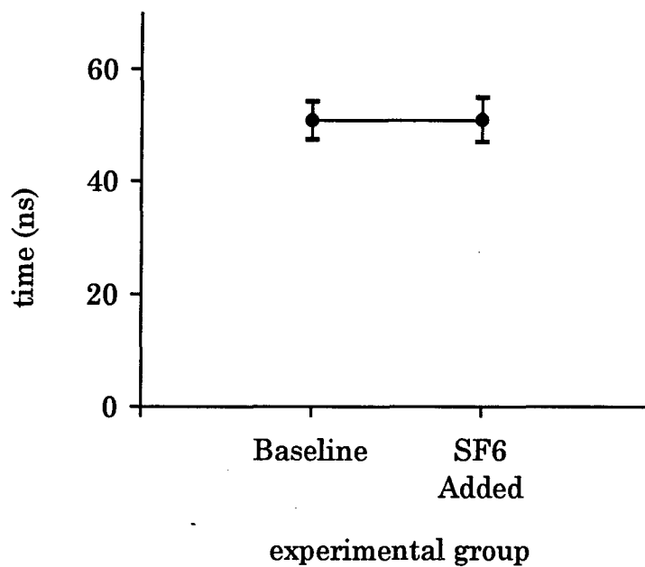
Figure 4-22. Effective time ( \tau_{eff} ) with SF 6 added (second series).
