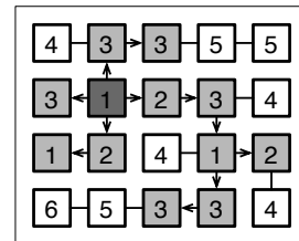
Traversal to i = 3
