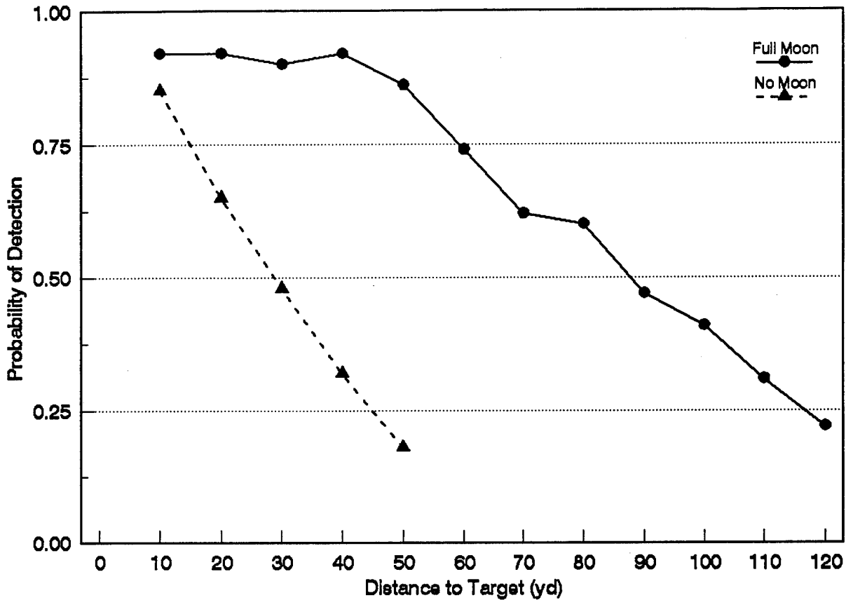
Figure 1. Probability of detection with unaided night vision (from Taylor, 1960). Probabilities were averaged over three observer and three target positions.
