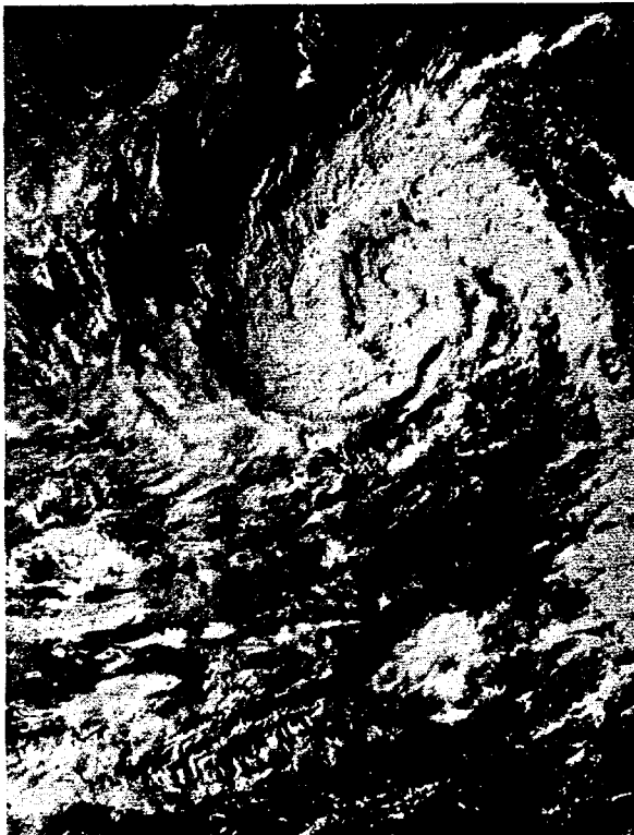
FIGURE 4-13. Alice as a 55 kt tropical storm 90 nm east-northeast of Catanduanes Island, 16 September 1975, 2205Z. (DMSP imagery)
