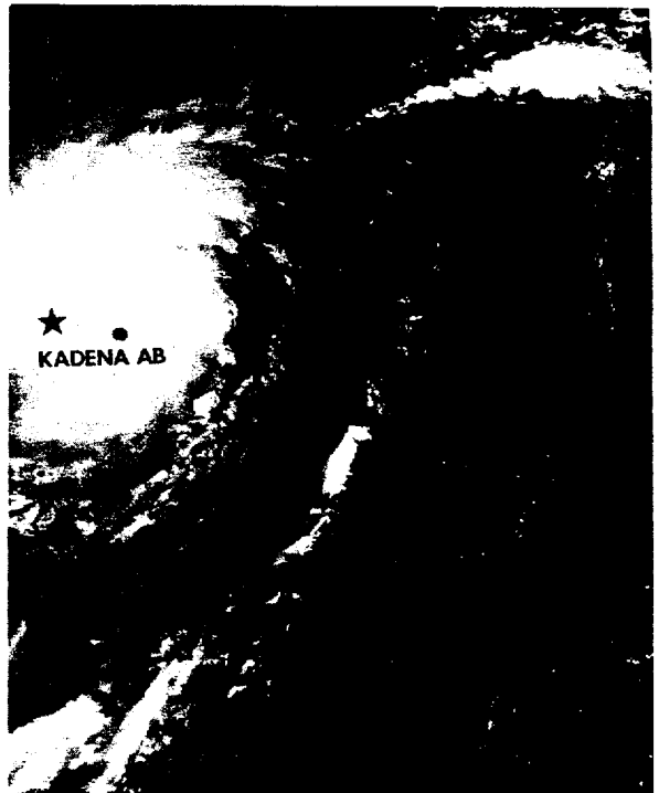
FIGURE 4-19. Typhoon Cora near 95 kt 115 nm east of Kadena AB, Okinawa, 4 October 1975, 0236Z. [DMSPI imagery]
