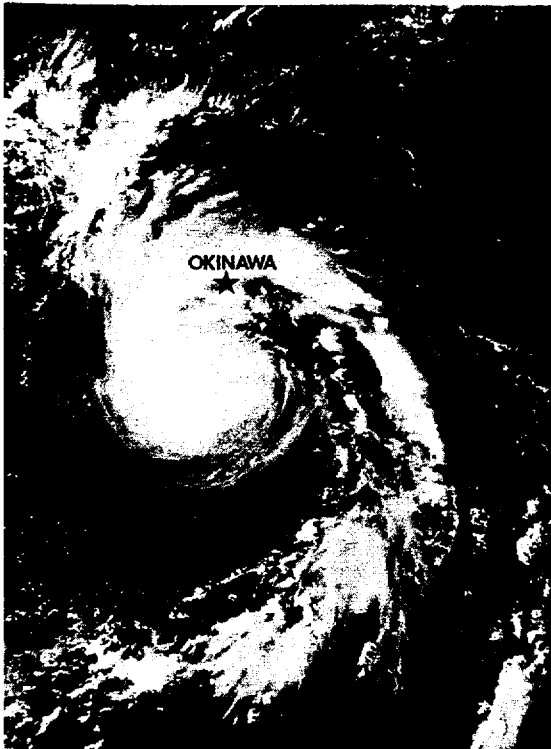
FIGURE 4-18. Cora just prior to attaining typhoon intensity 255 nm south-southeast of Okinawa, 3 October 1975, 0254Z. [DMSPI imagery]
