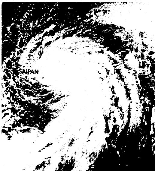
FIGURE 4-24. Ida just prior to achieving tropical storm intensity 255 nm east-northeast of Guam, 7 November 1975, 2224Z. [DMSP imagery]
