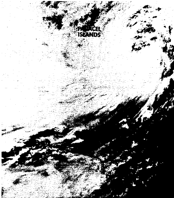
FIGURE 4-22. Flossie as a 45 kt tropical storm approximately 225 nm east-southeast of the Paracel Islands, 21 October 1975, 0032Z. (DMSP imagery)
