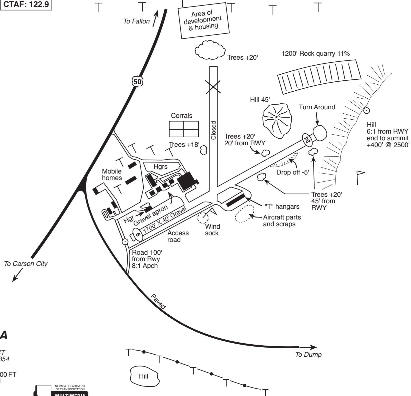
AIRPORT LAYOUT
