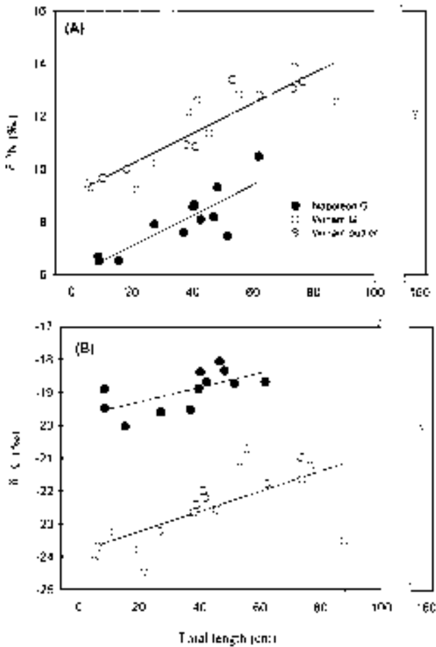
FIG. 6. \delta^{15}\text{N} (A) and \delta^{13}\text{C} (B) values in Nile perch versus their total length. The dotted outlier in each graph represents a very large Nile perch (TL = 158 cm) which was not included in the regression calculations.
