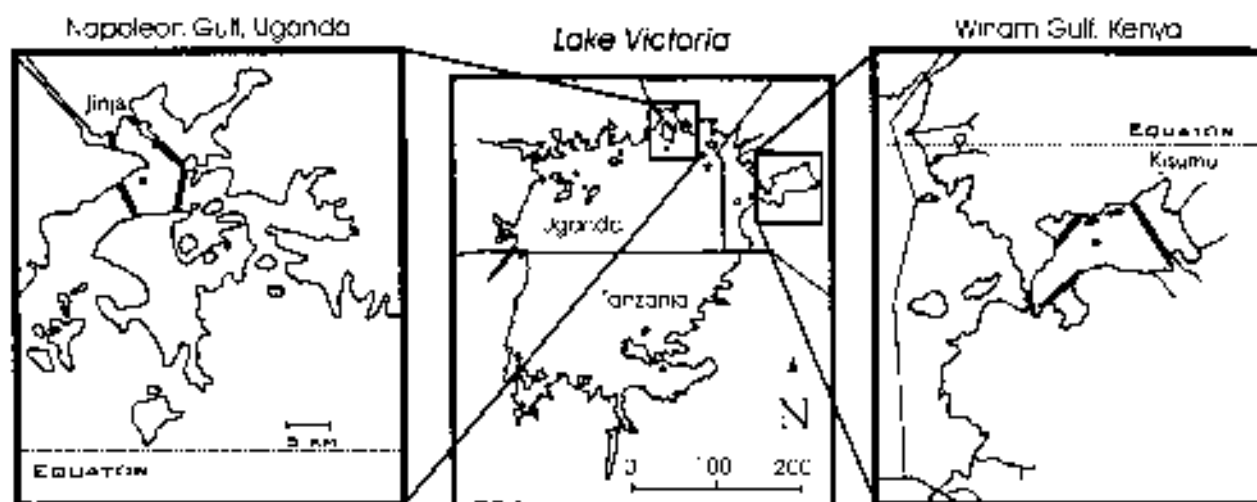
FIG. 1. Location of Napoleon Gulf (Uganda) and Winam Gulf (Kenya) in northern Lake Victoria, and the location of Lake Victoria in Africa. Regions bordered by thick lines indicate the sampling area.
