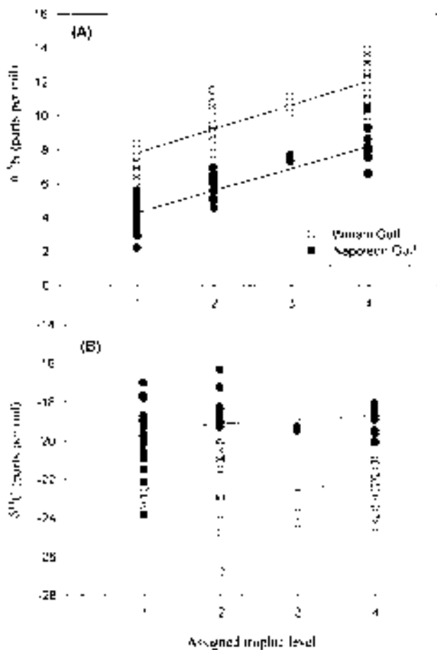
FIG. 4. \delta^{15}\text{N} (A) and \delta^{13}\text{C} (B) values of selected fish and Caridina versus their assigned numeric trophic position.
