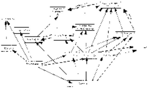
FIG. 7. A schematic food-web diagram of the food web structure based on stable isotope data from Napoleon and Winam Gulfs, Lake Victoria. The thin solid arrows demonstrate the energy flow from important dietary items to consumers. Dotted arrows indicate occasional dietary sources that are not isotopically important but are found in stomach contents of the predator fish. Dietary shifts from young to adult to very large adult Nile perch and for Nile tilapia are indicated.
