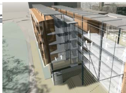
Left: Elevated view of the glazed walkways between the two building elements
