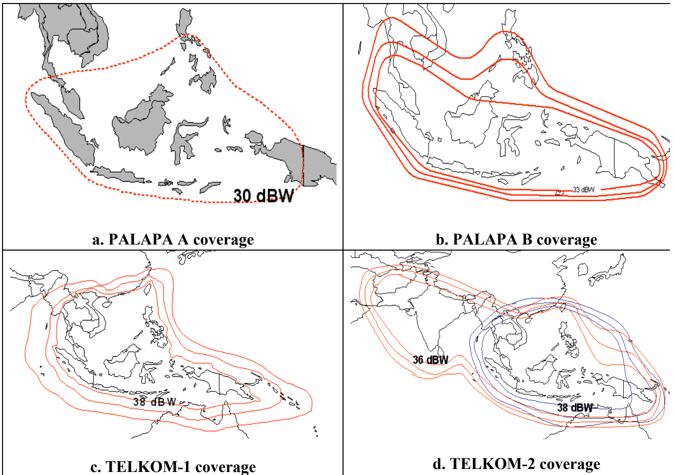
Figure 2. Coverage of PALAPA A, PALAPA B, TELKOM-1 and TELKOM-2
