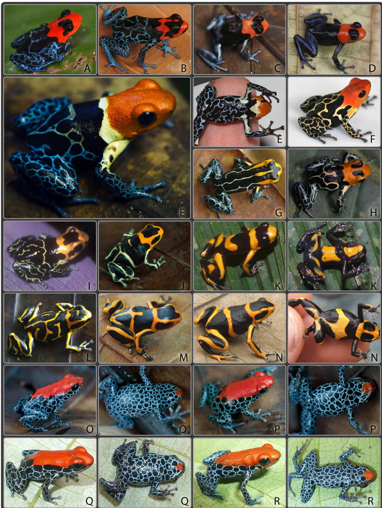
FIGURE 15. Ranitomeya Plate 3. reticulata group: A–D: Ranitomeya benedicta (all from Peru); A–B: Shucushuyacu, Loreto (1Φ); C–D: Pampa Hermosa, Loreto. E–L: Ranitomeya fantastica (all from Peru); E: Yurimaguas, Loreto; F: near Yumbatos, San Martin; G: Pongo de Cainarachi, San Martin (Ω); H: Cainarachi Valley, San Martin (Ω); I: San Antonio, San Martin (KS); J: Tarapoto, San Martin (Ω); K: Santa María de Nieva, Loreto (K.-H. Jungfer, 1Φ); L: Lower Huallaga Canyon, San Martin (Ω). M & N: Ranitomeya summersi (all from San Martin, Peru); M: Chazuta (3Φ); N: Sauce (Ω). O–R: Ranitomeya reticulata (all from Loreto, Peru); O–P: Iquitos (Ω); Q: Puerto Almendras (PPP); R: Upper Rio Itaya (PPP). (nΦ= number of individual in phylogeny, Ω = population sampled in phylogeny).
