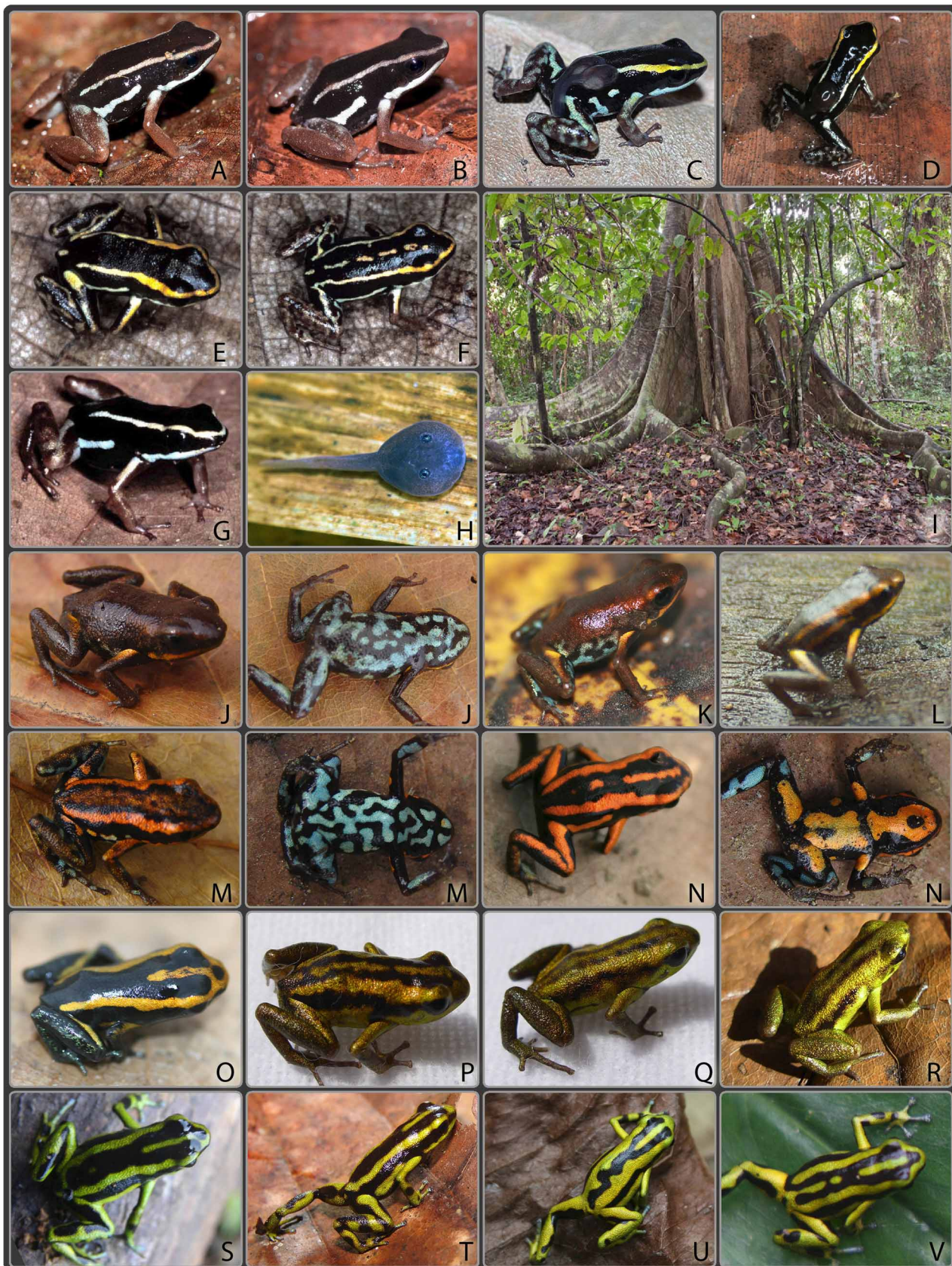
FIGURE 5. Andinobates Plate 1. minutus group: A–G: Andinobates claudiae and habitat (all from Bocas del Toro, Panama. Photos T. Ostrowski); A & B: Buena Esperanza; C–F: Isla Colon; G: Cerro Brujo; H: tadpole in phytotelm; I: habitat in Bocas del Toro, Panama. J–M: Andinobates minutus (all from Colombia. Photos DMV unless noted): J & K: Buenaventura, Valle del Cauca; L: Quibdó, Chocó; M: Baudó, Chocó (photo J. Mejía-Vargas). fulguritus group: N–V: Andinobates fulguritus (all from Colombia, photos DMV unless noted): N: Baudó, Chocó (photo J. Mejía-Vargas); O: Playa de Oro, Chocó (type locality); P–R: Uraba, Chocó. S–V: Anchicayá, Valle del Cauca. (nΦ = number of individual in phylogeny, Ω = population sampled in phylogeny).
