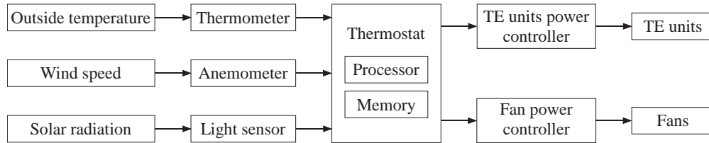
Figure 2. Thermostat and Sensors
