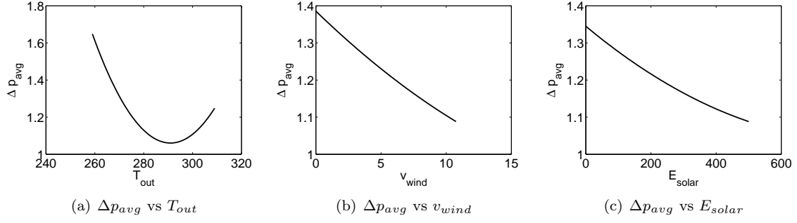
Figure 4. \Delta p_{avg} vs the Three Variables T_{out} , v_{wind} , and E_{solar}
