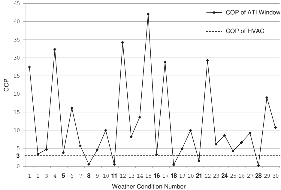
Figure 6. Values of COP_{ATI} under Different Weather Conditions
