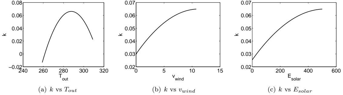
Figure 5. k vs the Three Variables T_{out} , v_{wind} , and E_{solar}
