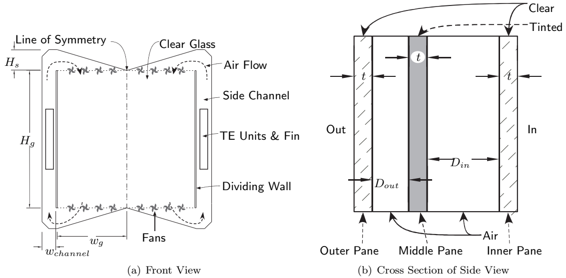
Figure 1. Schematic of the ATI Window
