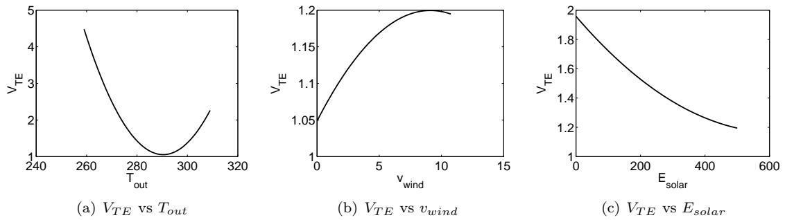
Figure 3. V_{TE} vs the Three Variables T_{out} , v_{wind} , and E_{solar}
