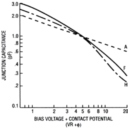
Figure 1. Tuning Varactor C-V Curves
