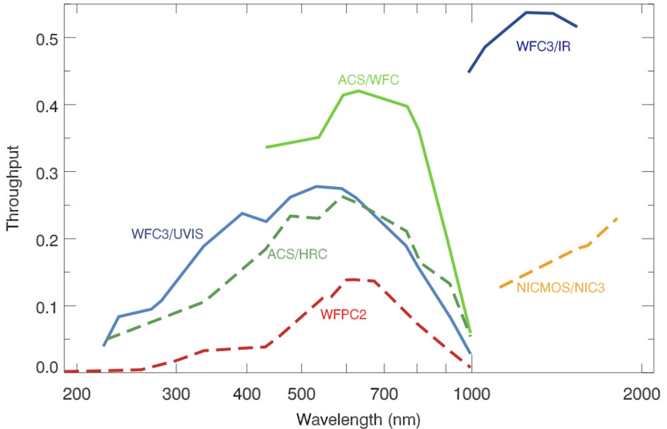
Figure 4.2: HST Total System Throughputs
