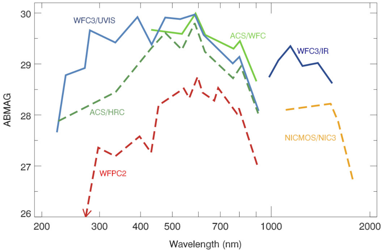
Figure 4.4: Point-Source Limiting Magnitude
