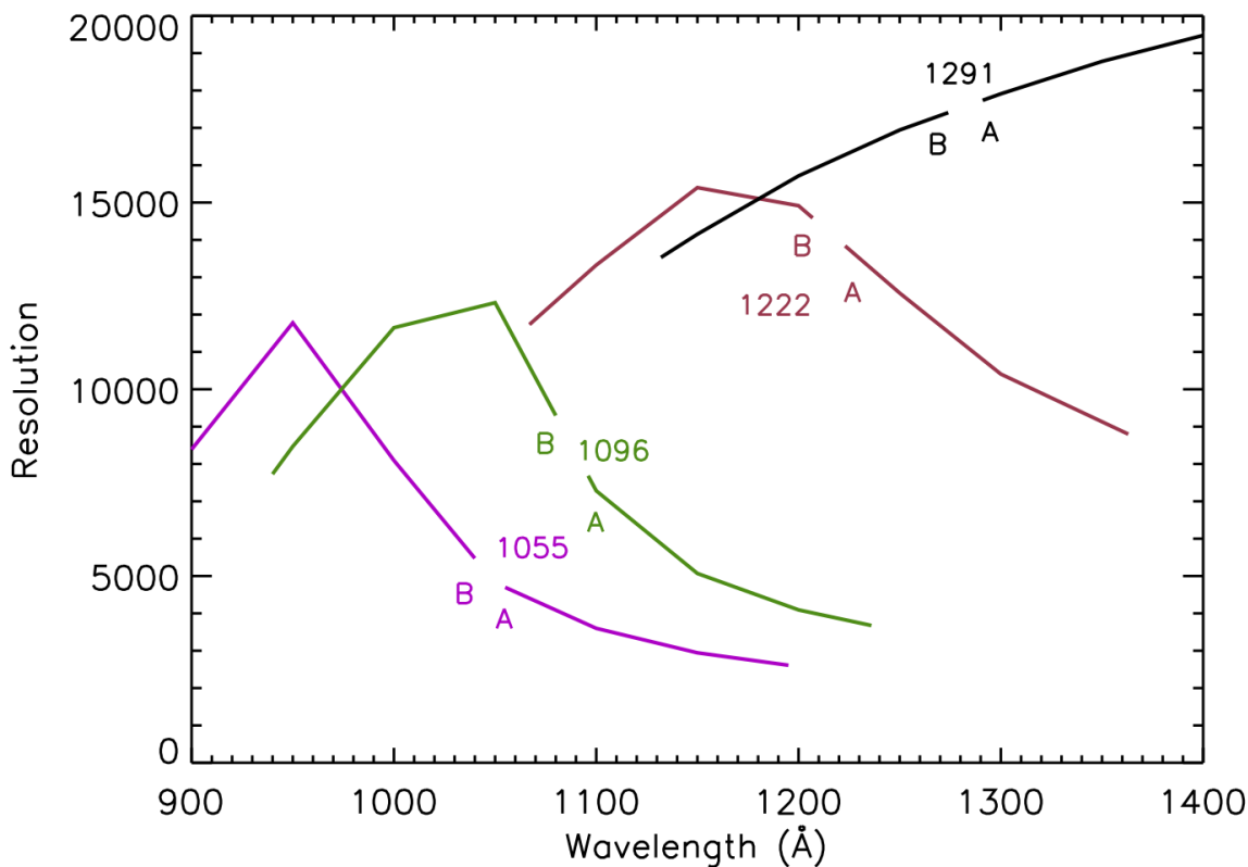
Figure 4.1: Predicted Resolution at LP2 as a Function of Wavelength for 1055 Å, 1096 Å, 1222 Å, and 1291 Å Central Wavelength Settings in Each COS FUV Segment
