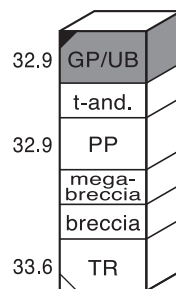
FIGURE 4—Three-dimensional depiction of the ignimbrite-based time-stratigraphic framework of the central Colorado volcanic field.
