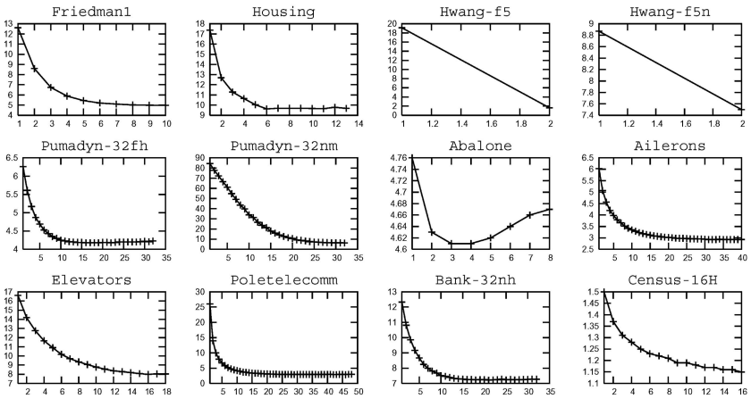
Fig. 2 Evolution of the error of Extra-Trees with K , on 12 classification and 12 regression problems.
