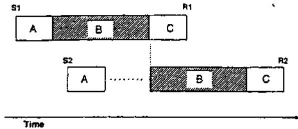
Figure 2. A central bottleneck model: The shaded portion of Task 2 cannot begin until the corresponding portion of Task 1 is complete. Other stages can operate in parallel, however. S = stimulus; R = response.
