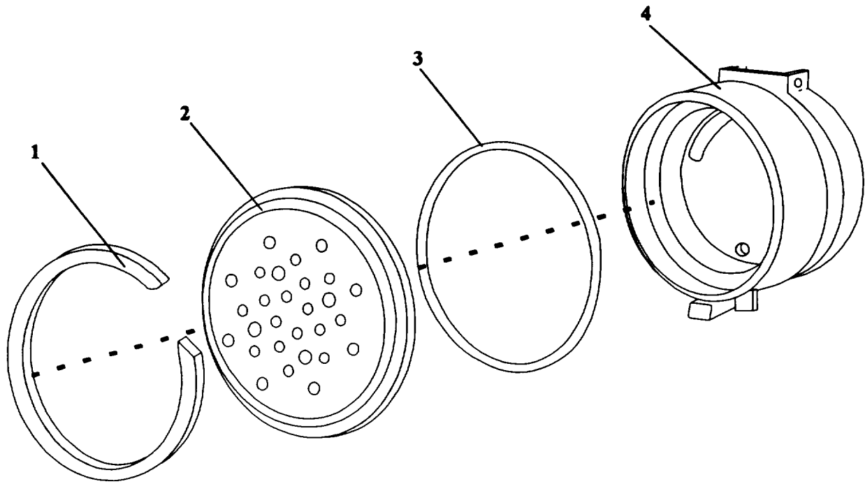
Figure C-6. Valve Cover Assembly
