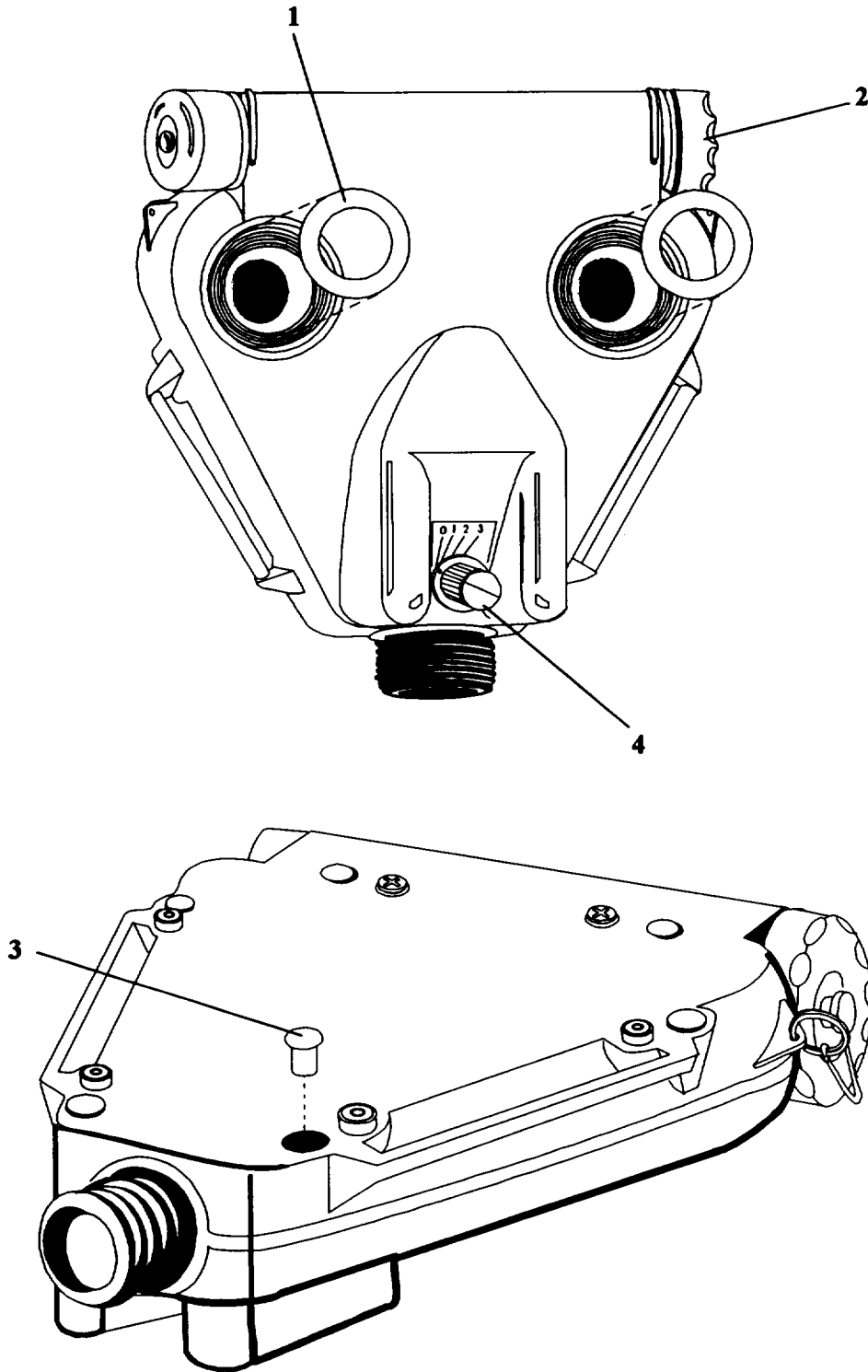
Figure C-9. Blower Assembly
