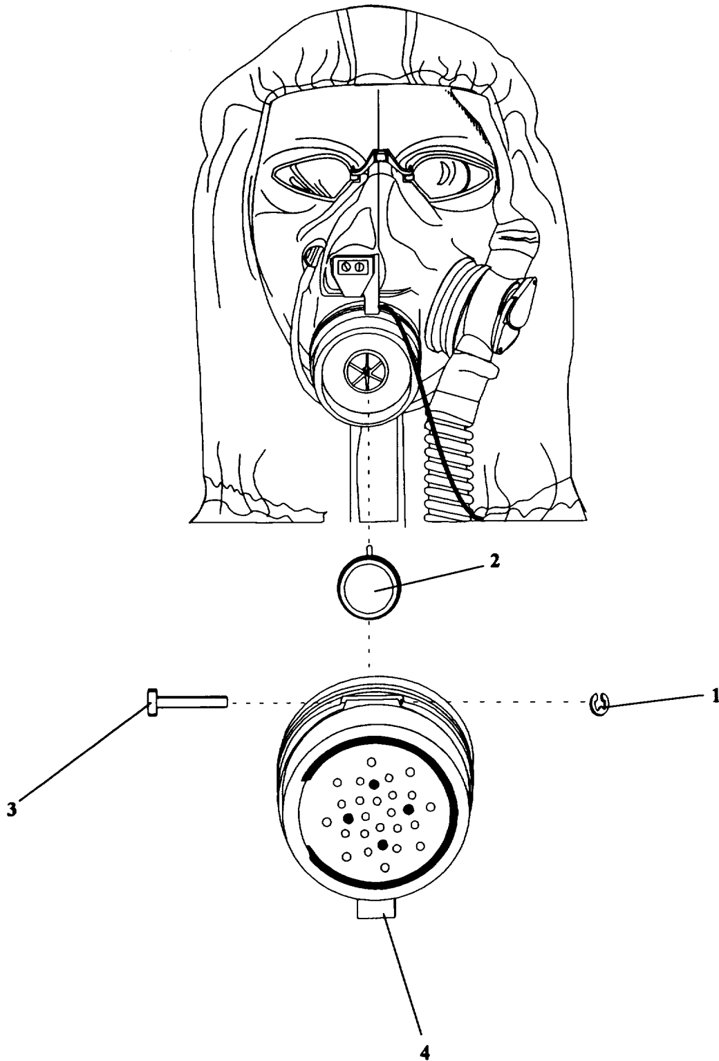
Figure C-5. Outlet Valve Assembly
