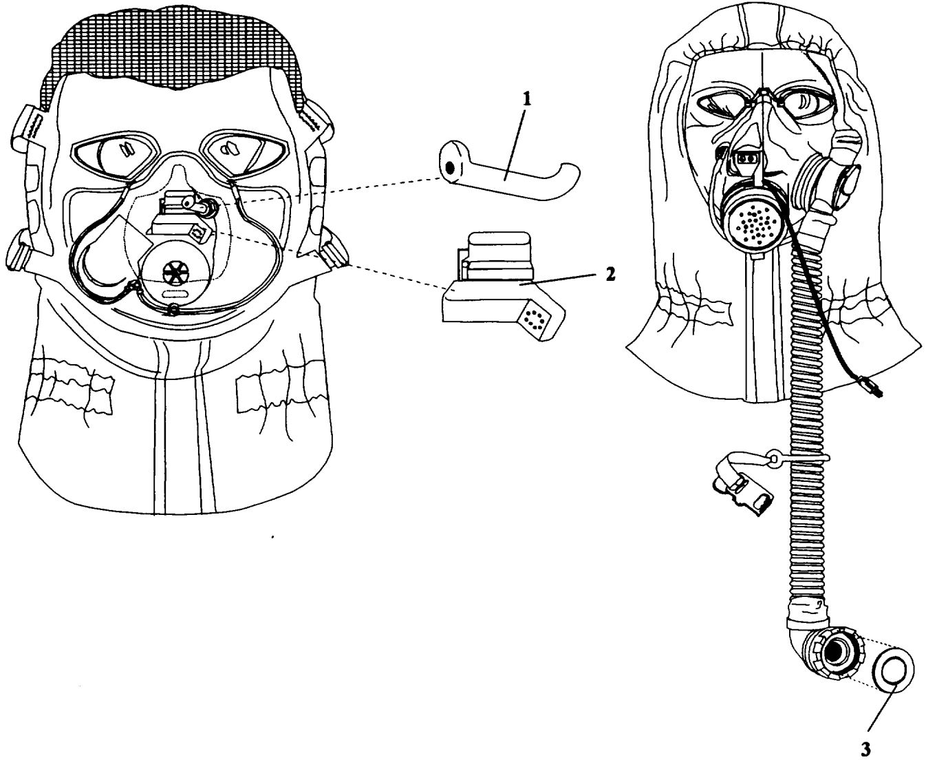
Figure C-3. Facepiece Assembly
