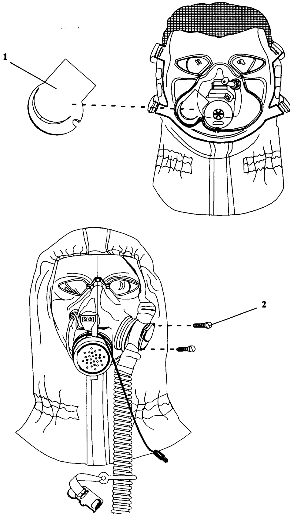
Figure C-4. Inlet Valve Assembly
