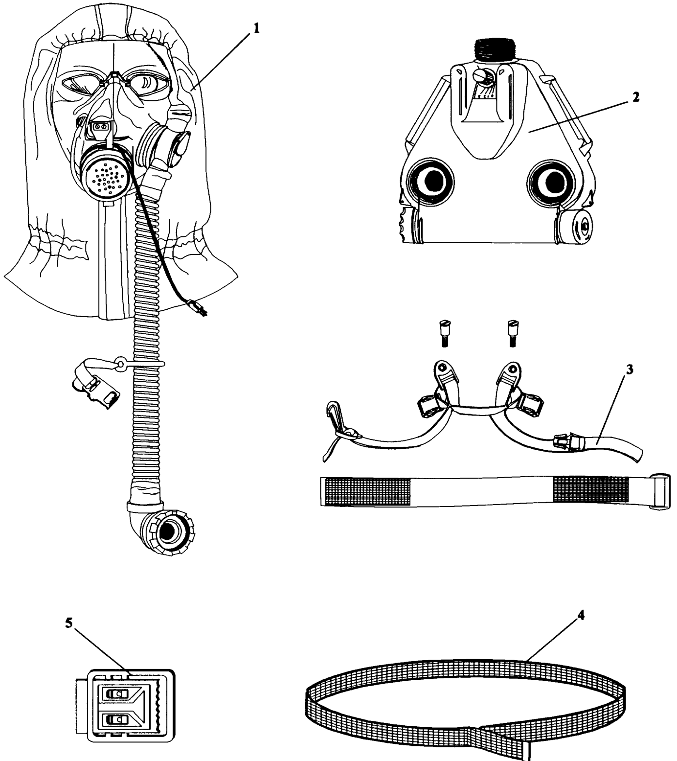
Figure C-1. Mask, Chemical-Biological Aircraft, Apache Aviator, M48
