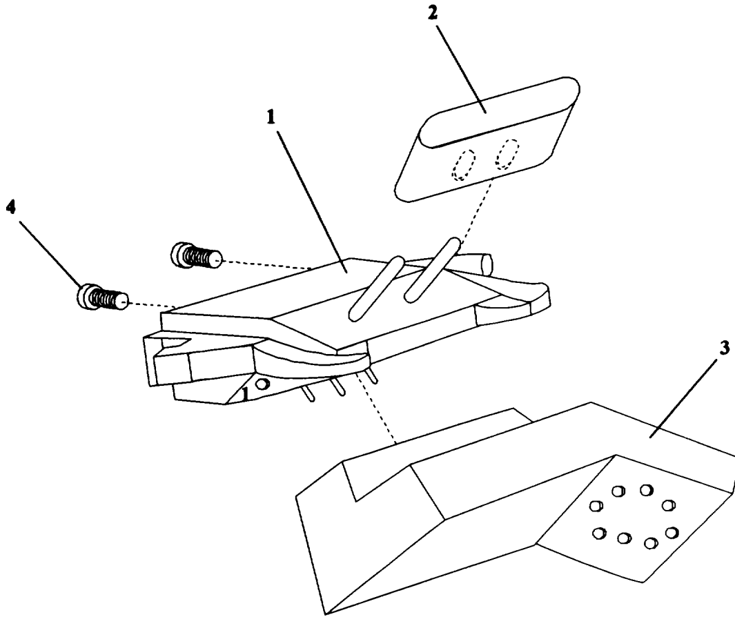
Figure C-7. Communications Assembly
