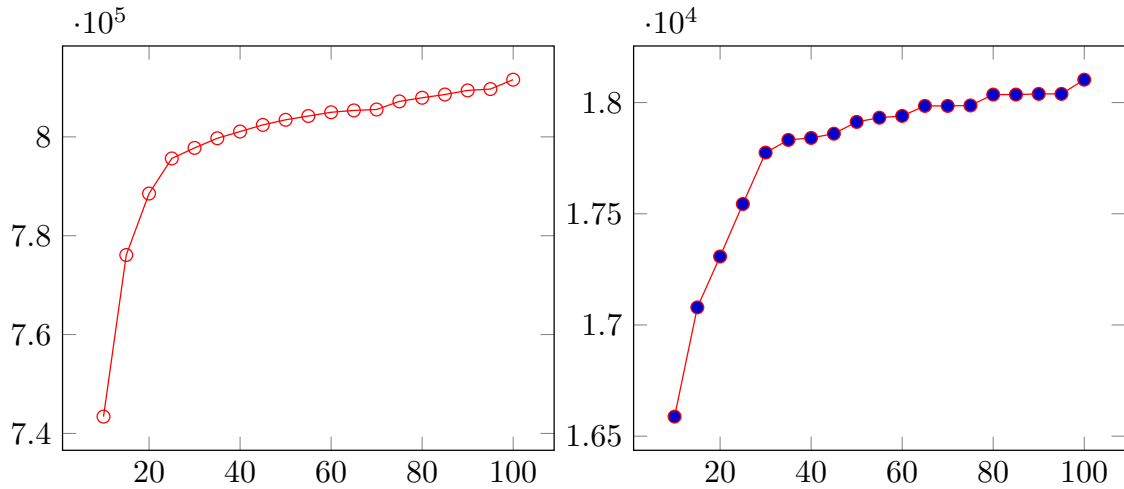
The number of terminating (left) and cycling (right) sequences starting below 10^6 plotted against the bound on the number of digits.
