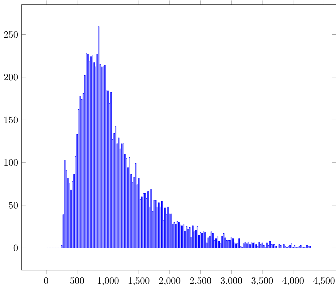
Distribution of lengths of main open sequences (the frequency of intervals of 25 lengths are shown)
