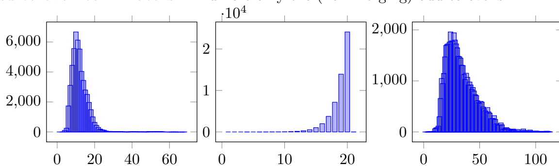
Lengths, heights, and volumes of odd-to-even terminating sequences.
