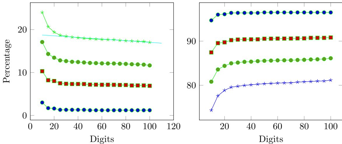
Comparing percentages of open (left) and terminating (right) sequences with starting values up to 10^m , for m = 3, 4, 5, 6 .
