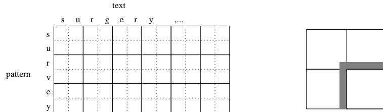
Figure 10: The Masek and Paterson algorithm partitions the dynamic programming matrix in cells ( r = 2 in this example). On the right, we shaded the entries of adjacent cells that influence the current one.
