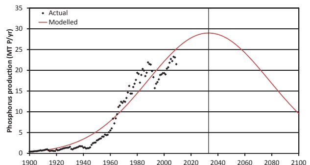
Figure 2.7 Indicative 'peak phosphorus' curve based on Cordell et al. (2009). This figure is presented so that the reader can follow the nature of the 'phosphorus debate' of recent years. Current analysis does not support the model estimates shown in this graph, with estimated P reserves and resources being considered to be much larger and longer lasting (for details see main text).
