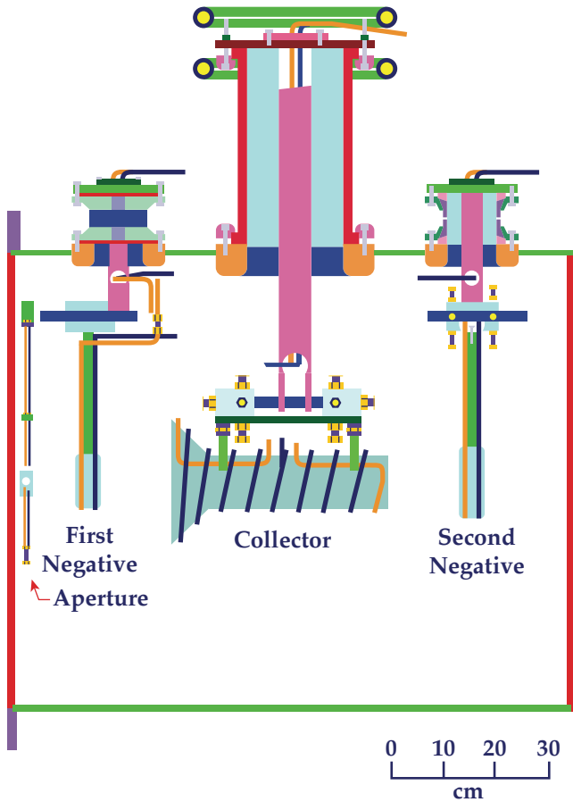
Figure 10 — The electrode assembly, showing electrodes, insulators, and electrode mountings. This view indicates the long dimension of the elliptical cross section in the horizontal direction. Other views would show a 90° rotation of the elliptical cross section.
