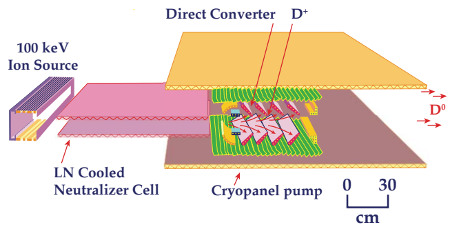
Figure 8 — A proposed 120-keV neutral injector system with a beam direct converter including cryopanel
