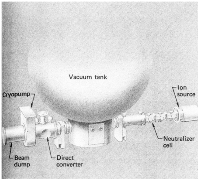
Figure 7 — Lawrence Berkeley Laboratory 120-keV test stand with the direct converter and cryopump
