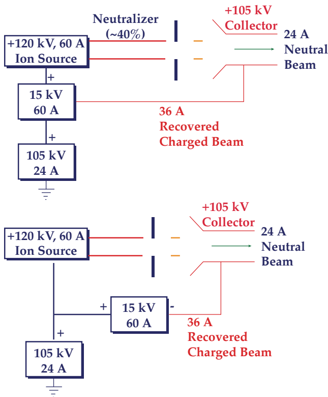
Figure 2 — Two examples of circuits to recirculate the recovered energy to supplement the acceleration power supply of ion sources for a device such as TFTR. In both designs, the total power supply requirement is 4.15 MW, assuming 40% neutralization efficiency for 120-kV D + . Compared to the total beam requirement of 60 A at 120 kV, the gross saving in acceleration power supplies is 3.05 MW (assuming 70% overall efficiency of beam direct conversion).
