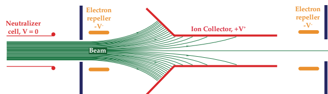
Figure 1 — Space-charge-controlled beam direct converter. In this version, the neutralizing cell is at ground potential and the potentials of the positive and negative electrodes are +V^+ and -V^- , respectively
