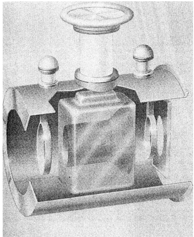
Figure 11 — The beam direct converter electrode assembly
