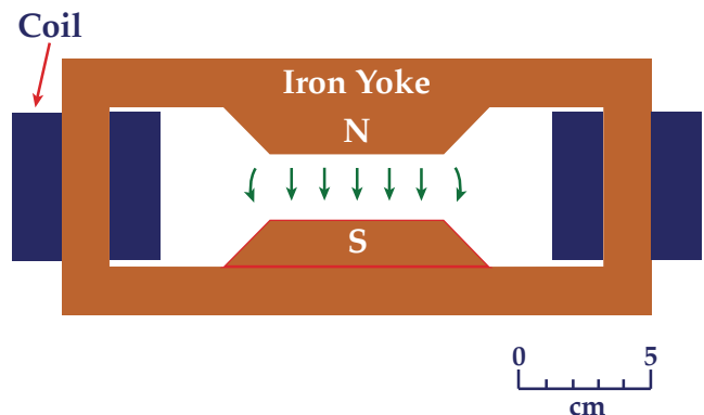
Figure 4 — The magnet used to produce a field perpendicular to the beam for magnetic electron suppression.
