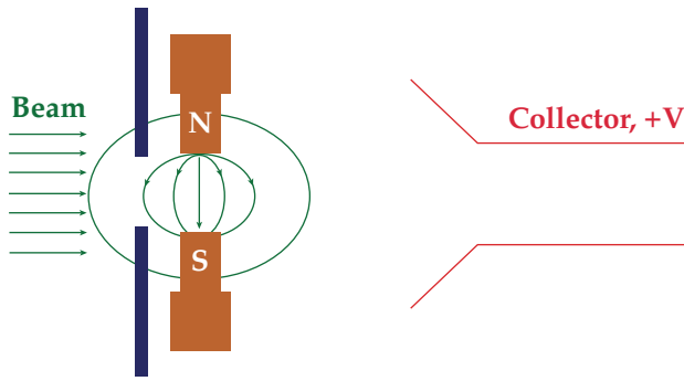
Figure 5(a) — The beam direct converter with a perpendicular field to suppress the electrons
