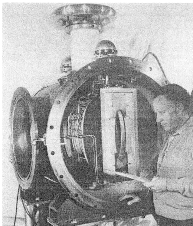
Figure 9 — The Lawrence Livermore Laboratory 120-keV beam direct converter showing the entrance aperture and the collector electrode. The high-voltage shield has been removed to show the water cooling systems.
