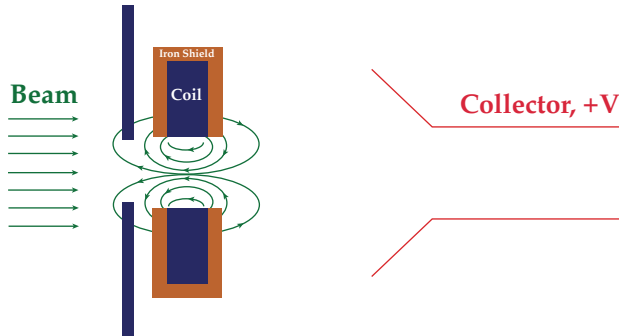
Figure 6(a) — Beam direct converter with a symmetrical magnetic electron suppressor.
