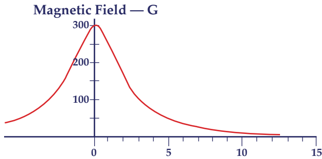
Figure 5(b) — Field strength along the axis
