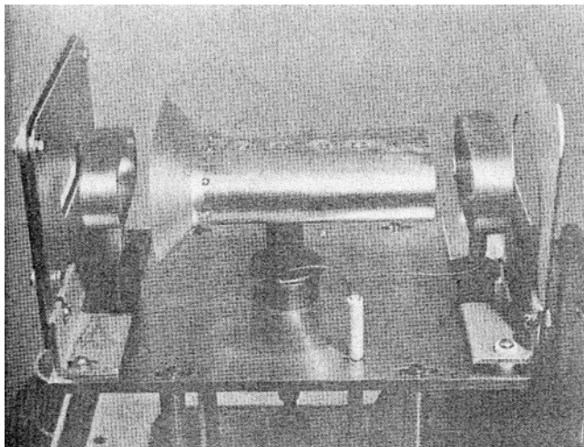
Figure 3 — A radiation-cooled, beam direct converter, operated at 15 kV and recovering 2 kW of energy. The electrodes are made of molybdenum
