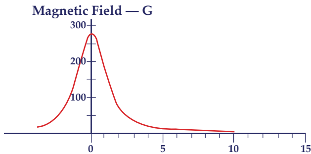
Figure 6(b) — Field strength along the axis.
