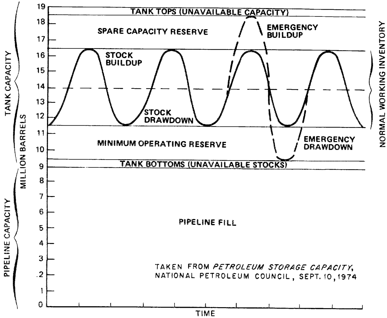
Fig. 8.2 Illustrative Operating Conditions Trans-Alaska Pipeline.
