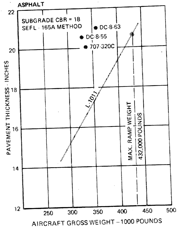
Fig. A.3 Runway Pavement Thickness for L-1011 Lockheed TriStar. SOURCE: Lockheed-California Company, Lockheed 1011 Technical and Operations Summary , COA 1323, Burbank, California, June 1971.
