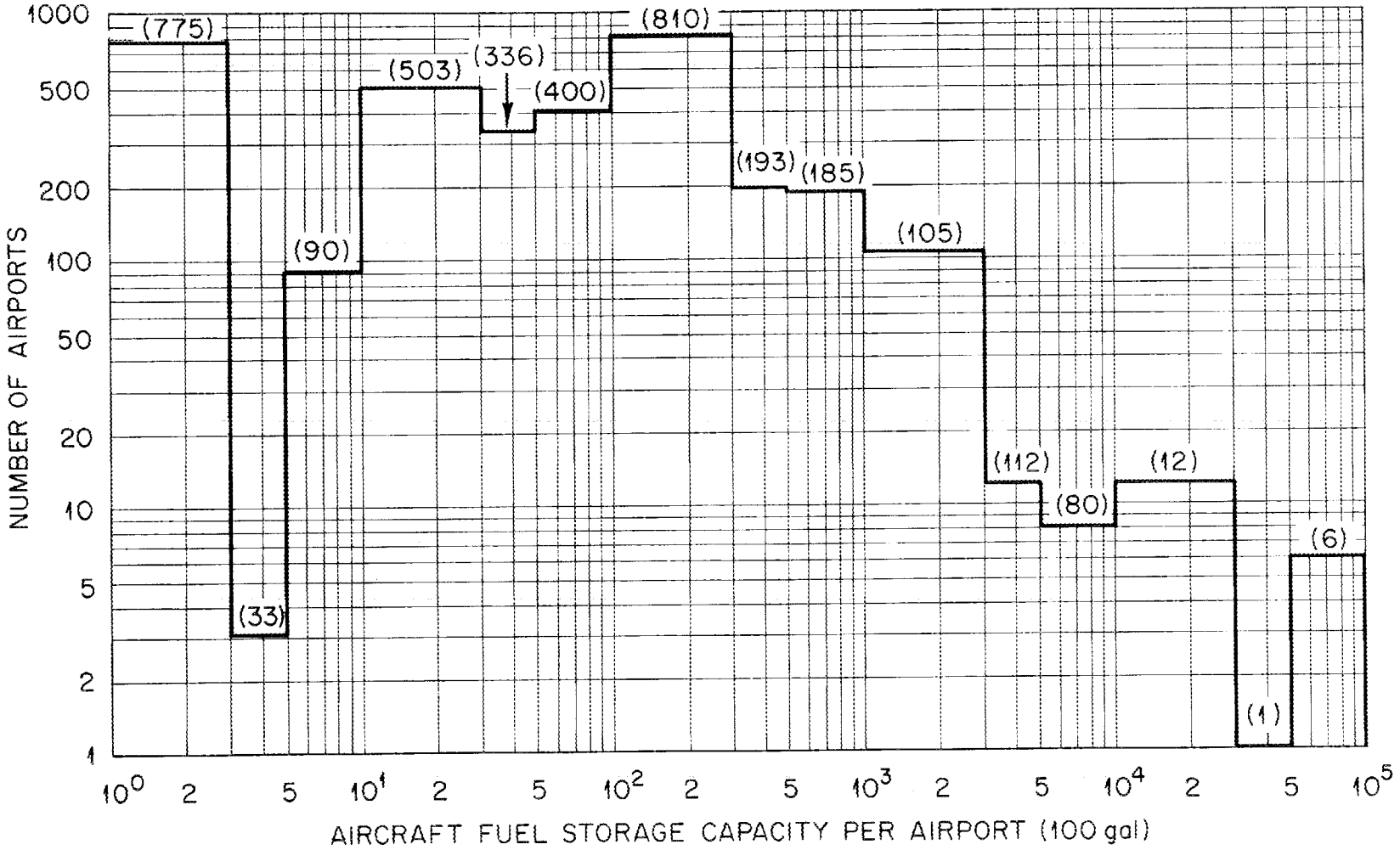
Fig. 7.4 Distribution of Fuel Storage Capacity.
