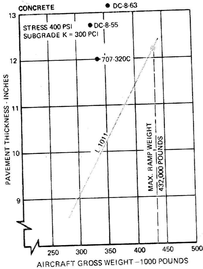
Fig. A.3 Runway Pavement Thickness for L-1011 Lockheed TriStar. SOURCE: Lockheed-California Company, Lockheed 1011 Technical and Operations Summary , COA 1323, Burbank, California, June 1971.
