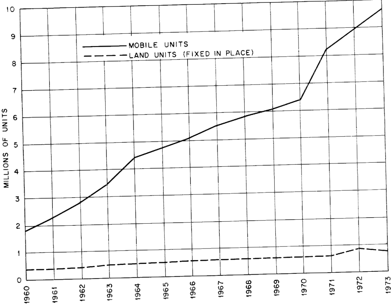
Fig. 5.3 Total Authorized Radio Transmitters, 1960-1973.
