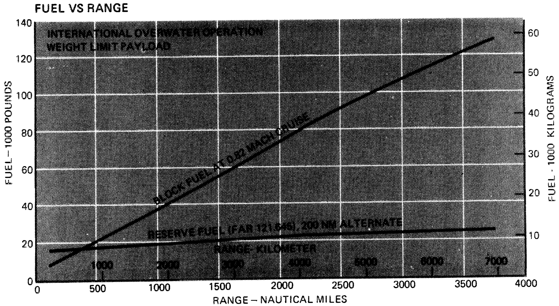
Fig. A.2 Fuel Requirements for the L-1011 Lockheed TriStar Aircraft. SOURCE: Lockheed-California Company, Lockheed 1011 Technical and Operations Summary , COA 1323, Burbank, California, June 1971.
