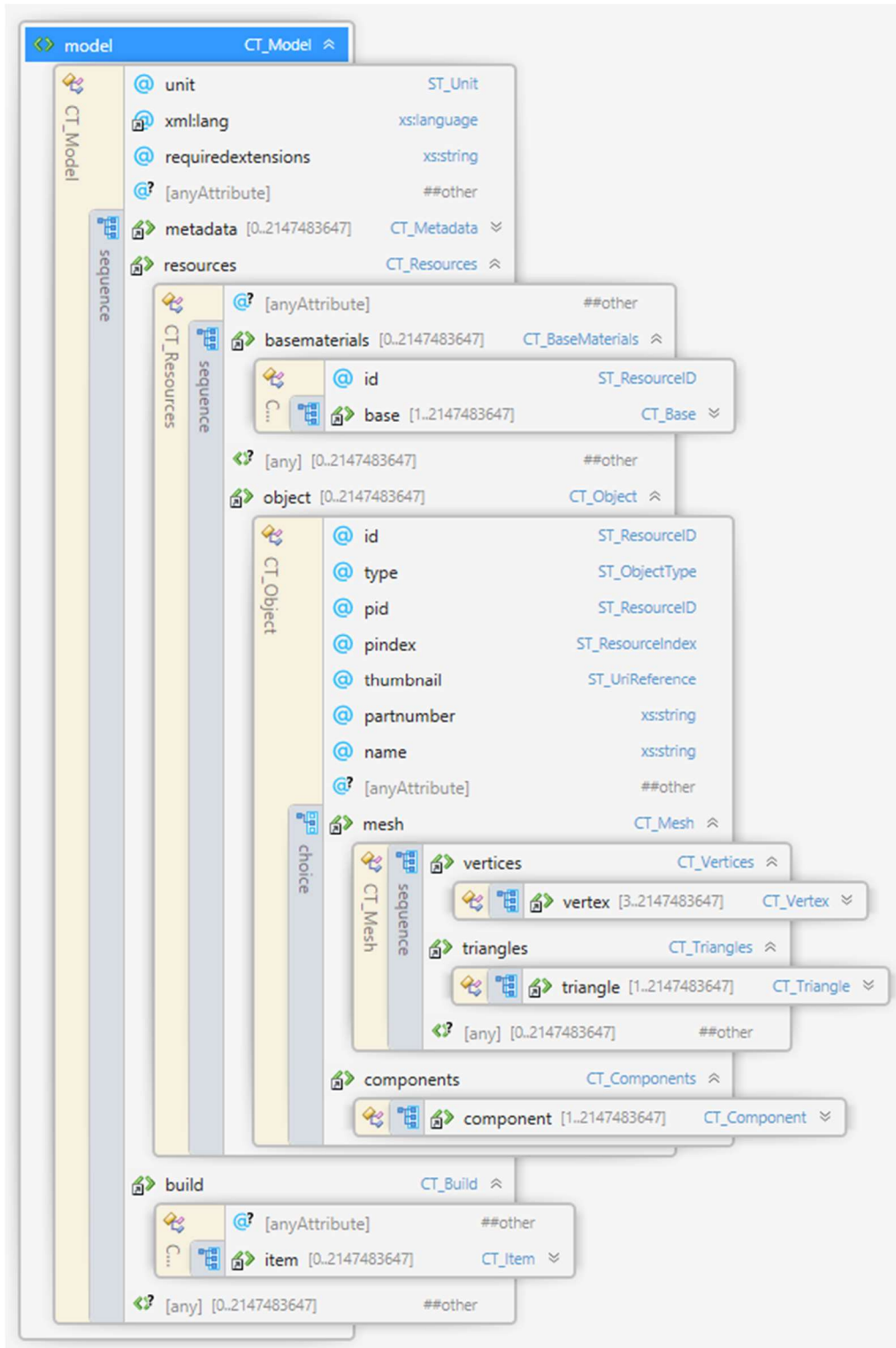
Figure 3-1: Overview of model XML structure of 3MF
