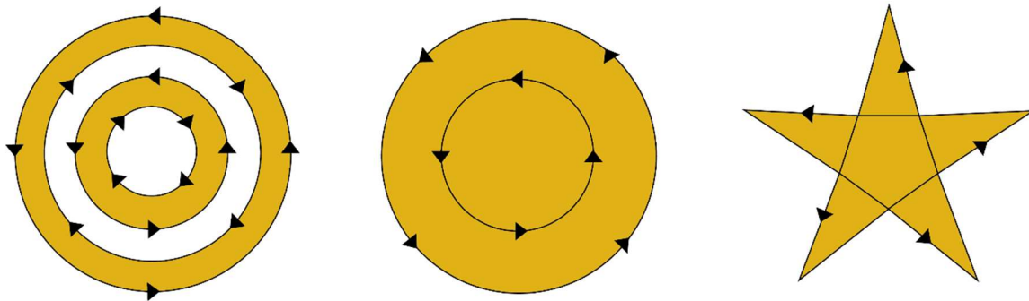
Figure 4–3. Fill using Positive algorithm
