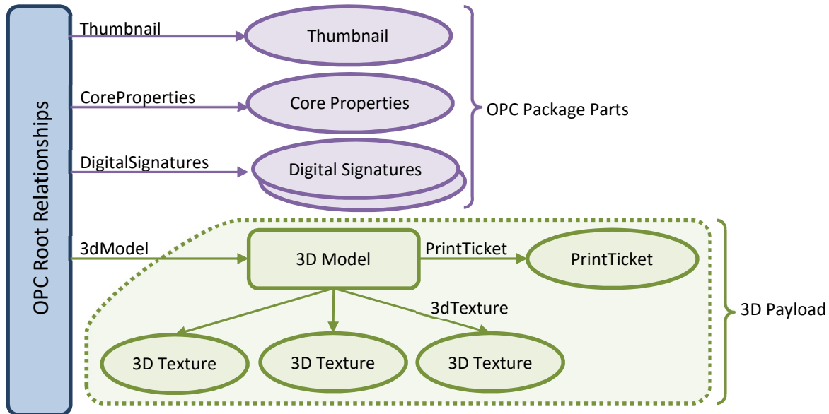
Figure 2–1. A typical 3MF Document
