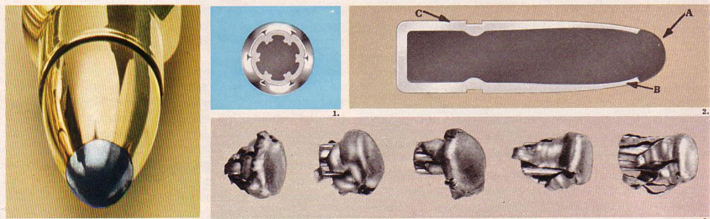
1. Here's Power-Point's inner secret: six scientifically determined notches for controlled expansion.
