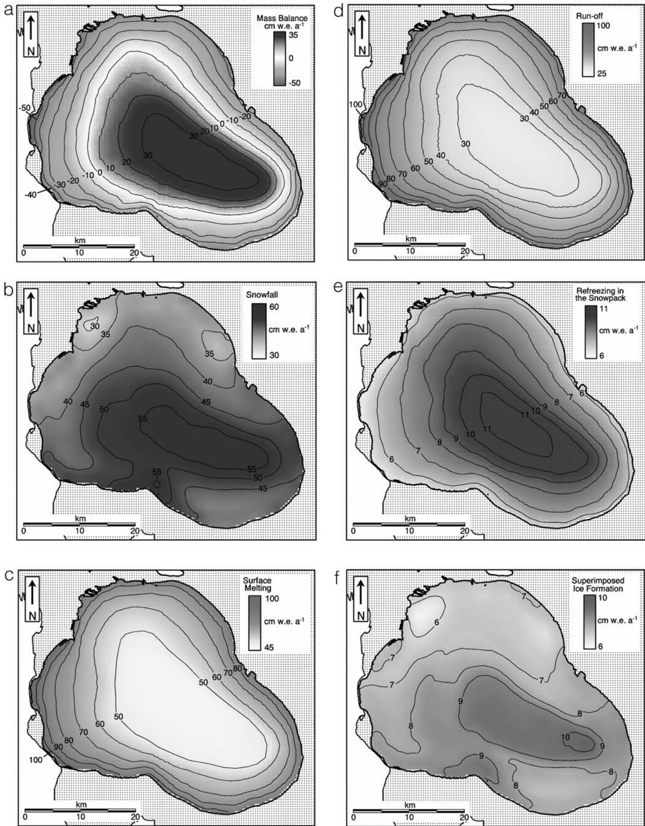
FIGURE 10. (a) Modeled mass balance of the Vavilov Ice Cap under the reference climate. Contours are at 10 cm w.e. a -1 intervals. (b) Modeled snowfall on the Vavilov Ice Cap under the reference climate. Contours are at 5 cm w.e. a -1 intervals. (c) Modeled surface melting of the Vavilov Ice Cap under the reference climate. Contours are at 10 cm w.e. a -1 intervals. (d) Modeled meltwater runoff from the Vavilov Ice Cap under the reference climate. Contours are at 10 cm w.e. a -1 intervals. (e) Modeled refreezing in the snowpack on the Vavilov Ice Cap under the reference climate. Contours are at 1 cm w.e. a -1 intervals. (f) Modeled superimposed ice formation on the Vavilov Ice Cap under the reference climate. Contours are at 1 cm w.e. a -1 intervals.
