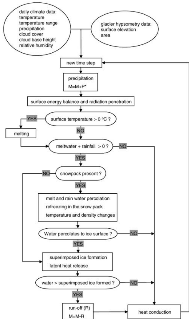
FIGURE 3. Schematic structure of the surface mass balance model. M denotes transient mass balance, P* is the precipitation rate, and R is runoff.
