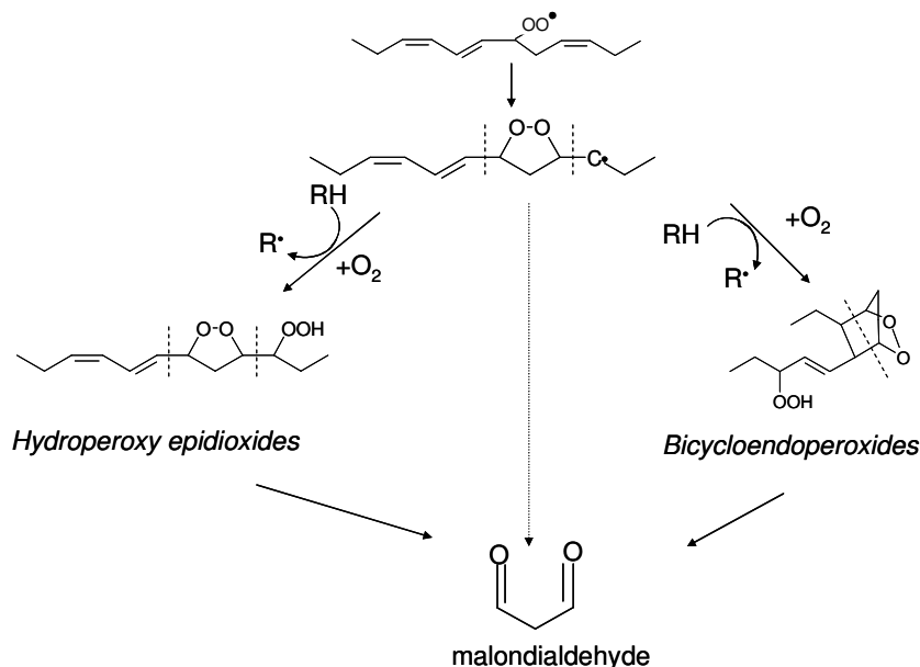
Figure 4.1.3.2-1 Formation of malondialdehyde from lipid peroxides (Frankel, 2005). Peroxyl radicals ( \text{LOO}\cdot ) of eicosapentaenoic acid (EPA) and docosapentaenoic acid (DHA) can be oxidised by cyclisation to hydroperoxy epidioxides and bicycloendoperoxides, which may be broken down to malondialdehyde as illustrated in the figure.
