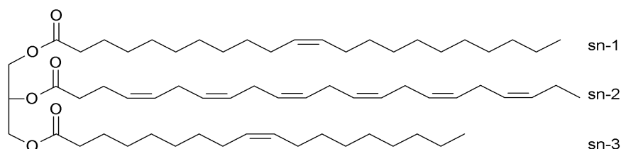
Figure 1.2.2-1 Structure of a triacylglycerol (TAG) molecule; three fatty acids esterified to the positions sn-1, sn-2 and sn-3
